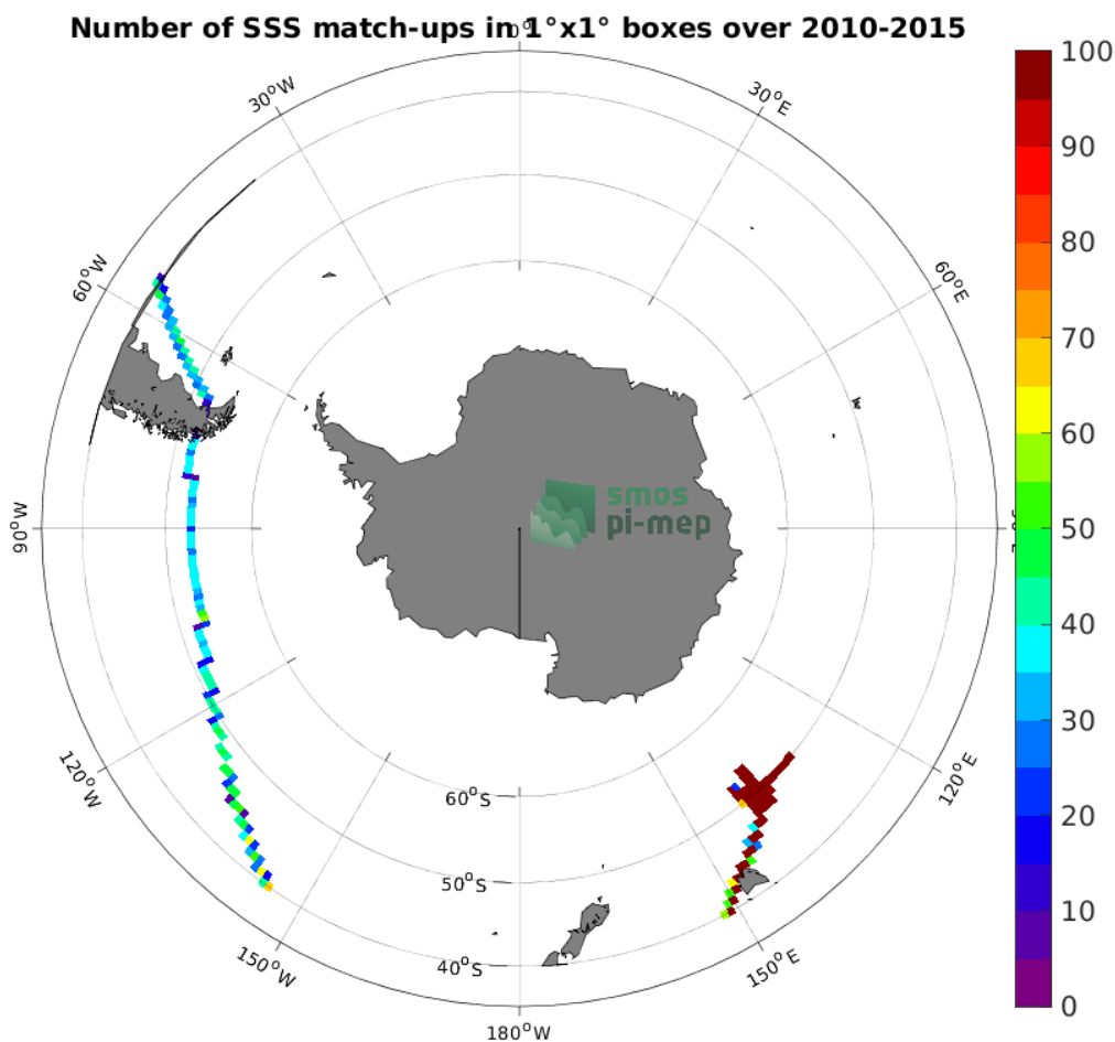
Figure 4: Number of SSS match-ups between TSG (GOSUD-Research-vessel) SSS and the SMOS SSS L4 v1 - Monthly (CMEMS-CNR) SSS product for the Roaring Forties and Furious Fifties Pi-MEP region over 1^\circ \times 1^\circ boxes and for the full satellite product period.
