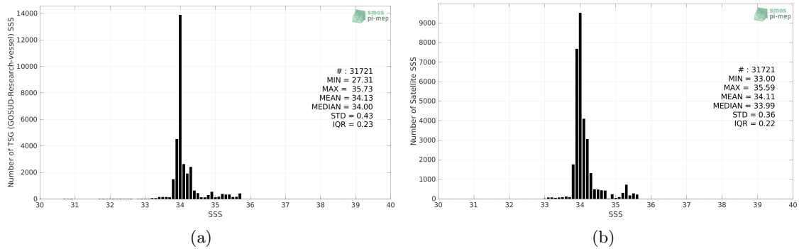
Figure 2: Histograms of SSS from TSG (GOSUD-Research-vessel) (a) and SMOS SSS L4 v1 - Monthly (CMEMS-CNR) (b) considering all match-up pairs per bins of 0.1 over the Roaring Forties and Furious Fifties Pi-MEP region and for the full satellite product period.
