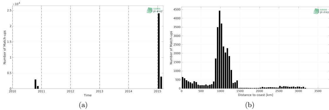
Figure 1: Number of match-ups between TSG (GOSUD-Research-vessel) and SMOS SSS L4 v1 - Monthly (CMEMS-CNR) SSS as a function of time (a) and as function of the distance to coast (b) over the Roaring Forties and Furious Fifties Pi-MEP region and for the full satellite product period.
