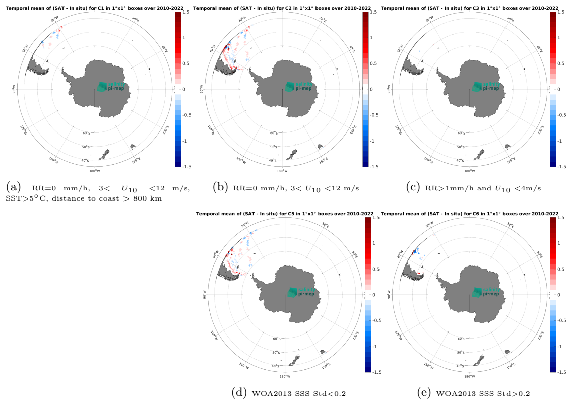
Figure 14: Temporal mean gridded over spatial boxes of size 1^\circ \times 1^\circ of \Delta SSS (SMOS SSS L4 v1 - Monthly (CMEMS-CNR) - TSG (CSIC-UTM)) for 5 different subdatasets corresponding to: RR=0 mm/h, 3 < U_{10} < 12 m/s, SST > 5^\circ\text{C} , distance to coast > 800 km (a), RR=0 mm/h, 3 < U_{10} < 12 m/s (b), RR > 1 mm/h and U_{10} < 4 m/s (c), WOA2013 SSS Std < 0.2 (d), WOA2013 SSS Std > 0.2 (e).
