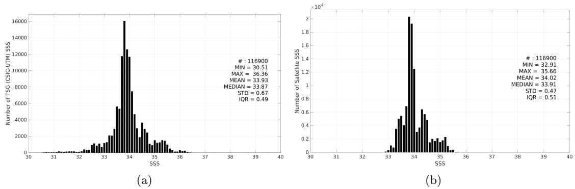
Figure 3: Histograms of SSS from TSG (CSIC-UTM) (a) and SMOS SSS L4 v1 - Monthly (CMEMS-CNR) (b) considering all match-up pairs per bins of 0.1 over the Roaring Forties and Furious Fifties Pi-MEP region and for the full satellite product period.
