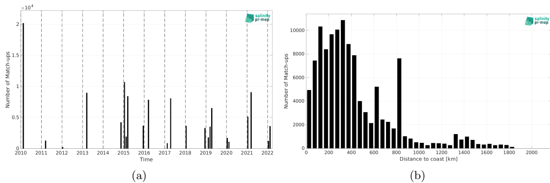
Figure 2: Number of match-ups between TSG (CSIC-UTM) and SMOS SSS L4 v1 - Monthly (CMEMS-CNR) SSS as a function of time (a) and as function of the distance to coast (b) over the Roaring Forties and Furious Fifties Pi-MEP region and for the full satellite product period.
