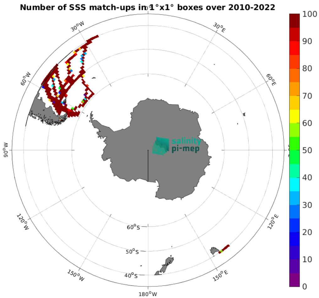
Figure 5: Number of SSS match-ups between TSG (CSIC-UTM) SSS and the SMOS SSS L4 v1 - Monthly (CMEMS-CNR) SSS product for the Roaring Forties and Furious Fifties Pi-MEP region over 1^\circ \times 1^\circ boxes and for the full satellite product period.
