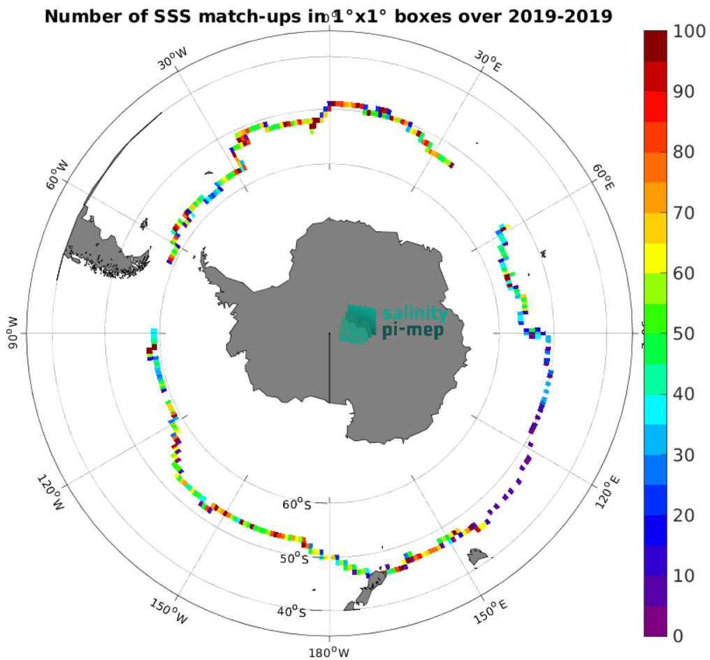
Figure 4: Number of SSS match-ups between Saildrone SSS and the SMOS SSS L4 v1 - Monthly (CMEMS-CNR) SSS product for the Roaring Forties and Furious Fifties Pi-MEP region over 1^\circ \times 1^\circ boxes and for the full satellite product period.
