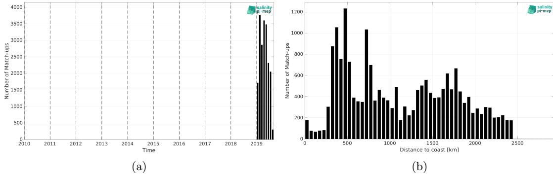
Figure 1: Number of match-ups between Saildrone and SMOS SSS L4 v1 - Monthly (CMEMS-CNR) SSS as a function of time (a) and as function of the distance to coast (b) over the Roaring Forties and Furious Fifties Pi-MEP region and for the full satellite product period.
