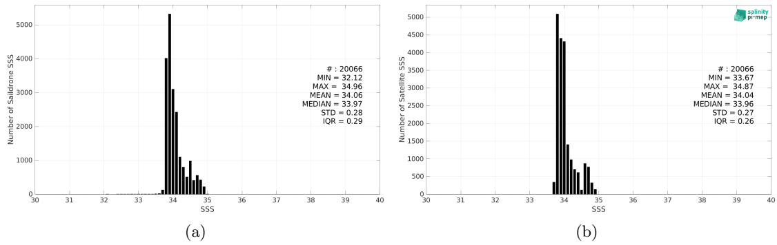
Figure 2: Histograms of SSS from Saildrone (a) and SMOS SSS L4 v1 - Monthly (CMEMS-CNR) (b) considering all match-up pairs per bins of 0.1 over the Roaring Forties and Furious Fifties Pi-MEP region and for the full satellite product period.
