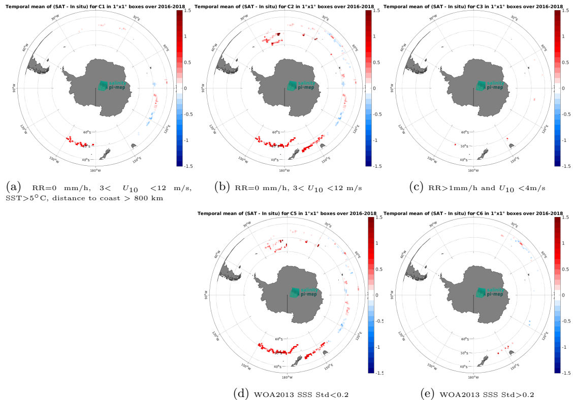
Figure 13: Temporal mean gridded over spatial boxes of size 1^\circ \times 1^\circ of \Delta SSS (SMOS SSS L4 v1 - Monthly (CMEMS-CNR) - Surface drifters) for 5 different subdatasets corresponding to:RR=0 mm/h, 3 < U_{10} < 12 m/s, SST > 5^\circ\text{C} , distance to coast > 800 km (a), RR=0 mm/h, 3 < U_{10} < 12 m/s (b), RR > 1 mm/h and U_{10} < 4 m/s (c), WOA2013 SSS Std < 0.2 (d), WOA2013 SSS Std > 0.2 (e).
