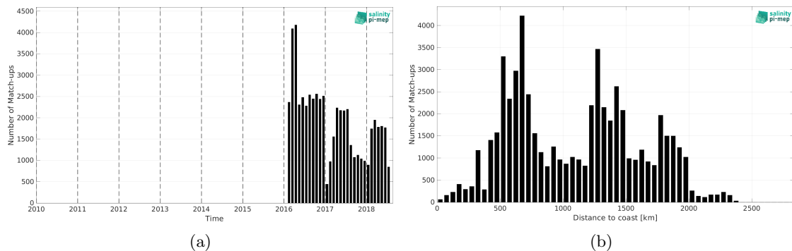
Figure 2: Number of match-ups between Surface drifters and SMOS SSS L4 v1 - Monthly (CMEMS-CNR) SSS as a function of time (a) and as function of the distance to coast (b) over the Roaring Forties and Furious Fifties Pi-MEP region and for the full satellite product period.
