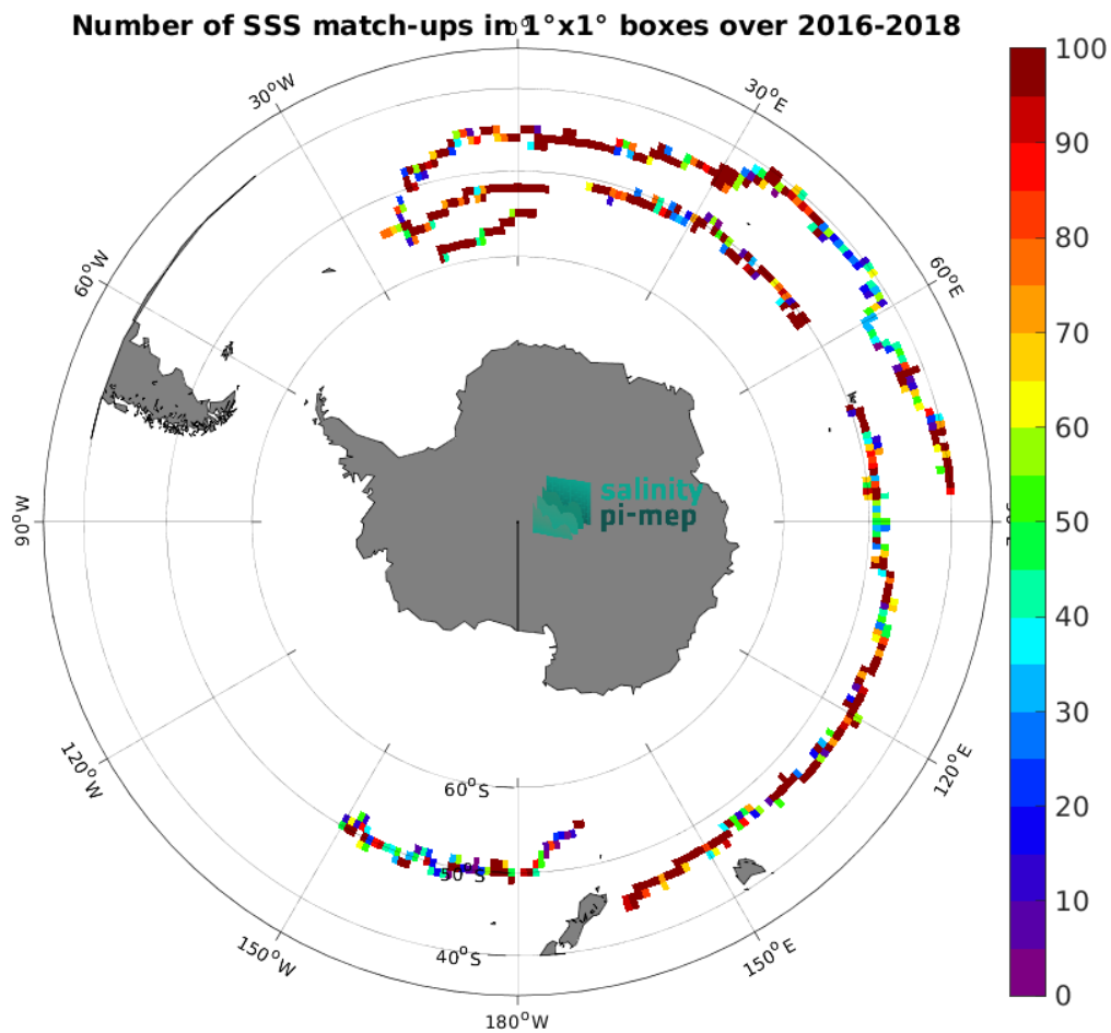
Figure 4: Number of SSS match-ups between Surface drifters SSS and the SMOS SSS L4 v1 - Monthly (CMEMS-CNR) SSS product for the Roaring Forties and Furious Fifties Pi-MEP region over 1^\circ \times 1^\circ boxes and for the full satellite product period.
