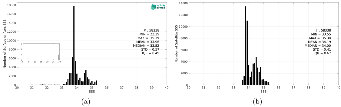
Figure 3: Histograms of SSS from Surface drifters (a) and SMOS SSS L4 v1 - Monthly (CMEMS-CNR) (b) considering all match-up pairs per bins of 0.1 over the Roaring Forties and Furious Fifties Pi-MEP region and for the full satellite product period.
