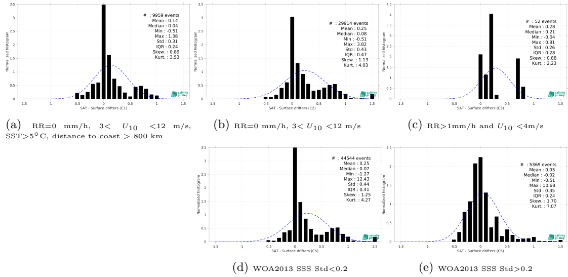
Figure 14: Normalized histogram of \Delta SSS (SMOS SSS L4 v1 - Monthly (CMEMS-CNR) - Surface drifters) for 5 different subdatasets corresponding to: RR=0 mm/h, 3 < U_{10} < 12 m/s, SST >5^{\circ} C, distance to coast > 800 km (a), RR=0 mm/h, 3 < U_{10} < 12 m/s (b), RR >1 mm/h and U_{10} < 4 m/s (c), WOA2013 SSS Std <0.2 (d), WOA2013 SSS Std >0.2 (e).
