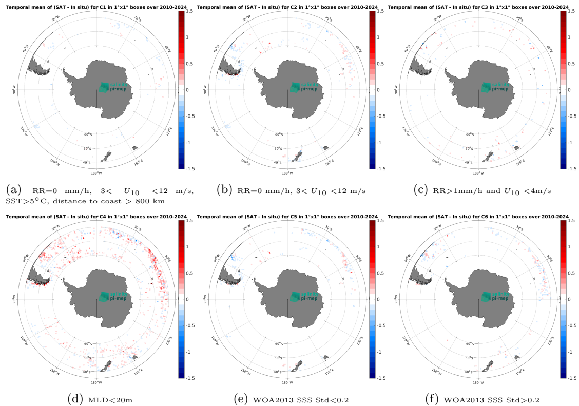
Figure 14: Temporal mean gridded over spatial boxes of size 1^\circ \times 1^\circ of \Delta SSS (SMOS SSS L4 v1 - Monthly (CMEMS-CNR) - Argo) for 6 different subdatasets corresponding to: RR=0 mm/h, 3 < U_{10} < 12 m/s, SST > 5^\circ\text{C} , distance to coast > 800 km (a), RR=0 mm/h, 3 < U_{10} < 12 m/s (b), RR > 1 mm/h and U_{10} < 4 m/s (c), MLD < 20 m (d), WOA2013 SSS Std < 0.2 (e), WOA2013 SSS Std > 0.2 (f).
