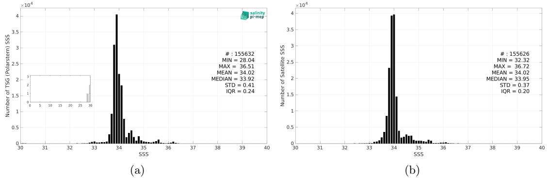
Figure 3: Histograms of SSS from TSG (Polarstern) (a) and SMOS SSS L4 v1 - Daily (CMEMS-CNR) (b) considering all match-up pairs per bins of 0.1 over the Roaring Forties and Furious Fifties Pi-MEP region and for the full satellite product period.
