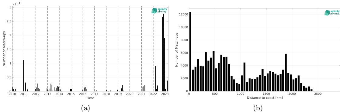
Figure 2: Number of match-ups between TSG (Polarstern) and SMOS SSS L4 v1 - Daily (CMEMS-CNR) SSS as a function of time (a) and as function of the distance to coast (b) over the Roaring Forties and Furious Fifties Pi-MEP region and for the full satellite product period.
