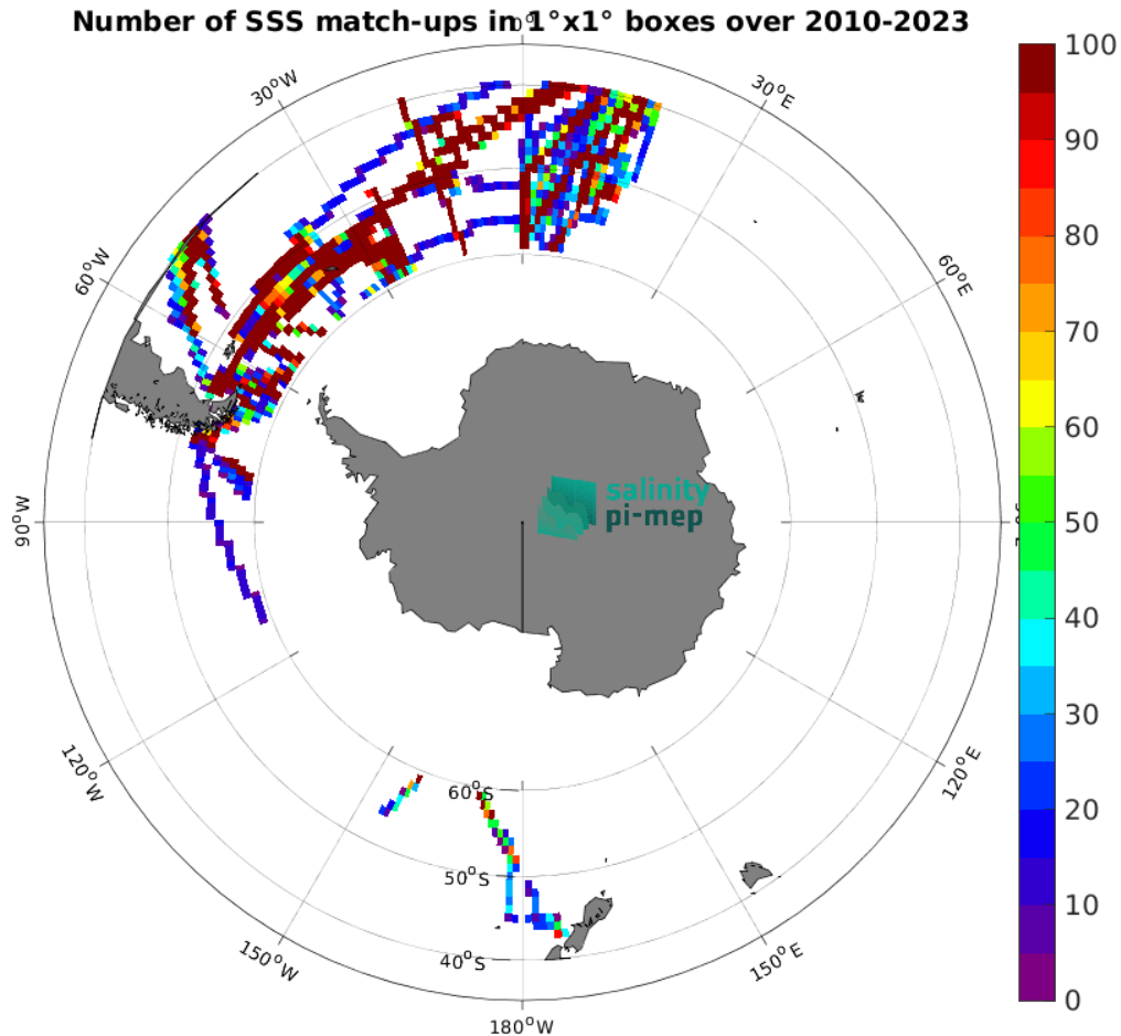
Figure 5: Number of SSS match-ups between TSG (Polarstern) SSS and the SMOS SSS L4 v1 - Daily (CMEMS-CNR) SSS product for the Roaring Forties and Furious Fifties Pi-MEP region over 1^\circ \times 1^\circ boxes and for the full satellite product period.
