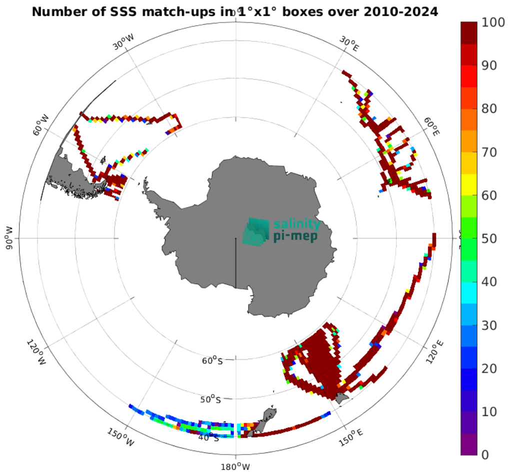
Figure 5: Number of SSS match-ups between TSG (LEGOS-DM) SSS and the SMOS SSS L4 v1 - Daily (CMEMS-CNR) SSS product for the Roaring Forties and Furious Fifties Pi-MEP region over 1^\circ \times 1^\circ boxes and for the full satellite product period.
