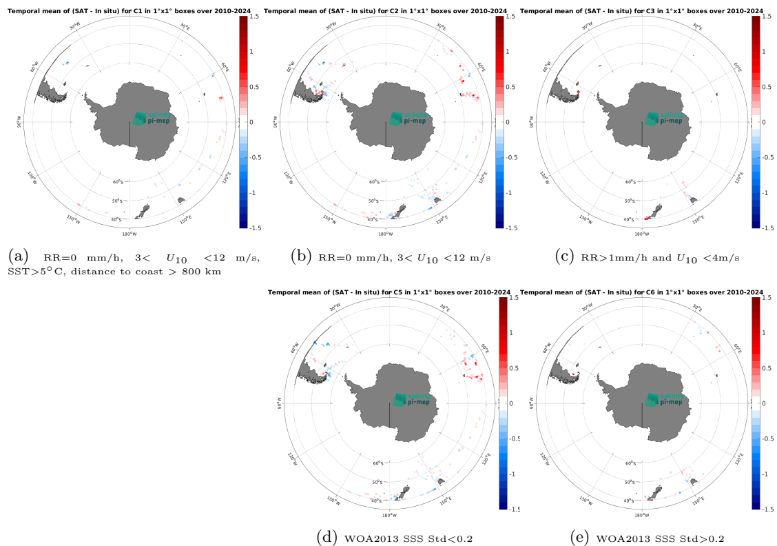
Figure 14: Temporal mean gridded over spatial boxes of size 1^\circ \times 1^\circ of \Delta\text{SSS} (SMOS SSS L4 v1 - Daily (CMEMS-CNR) - TSG (LEGOS-DM)) for 5 different subdatasets corresponding to:RR=0 mm/h, 3 < U_{10} < 12 m/s, SST > 5°C, distance to coast > 800 km (a), RR=0 mm/h, 3 < U_{10} < 12 m/s (b), RR > 1mm/h and U_{10} < 4 m/s (c), WOA2013 SSS Std < 0.2 (d), WOA2013 SSS Std > 0.2 (e).
