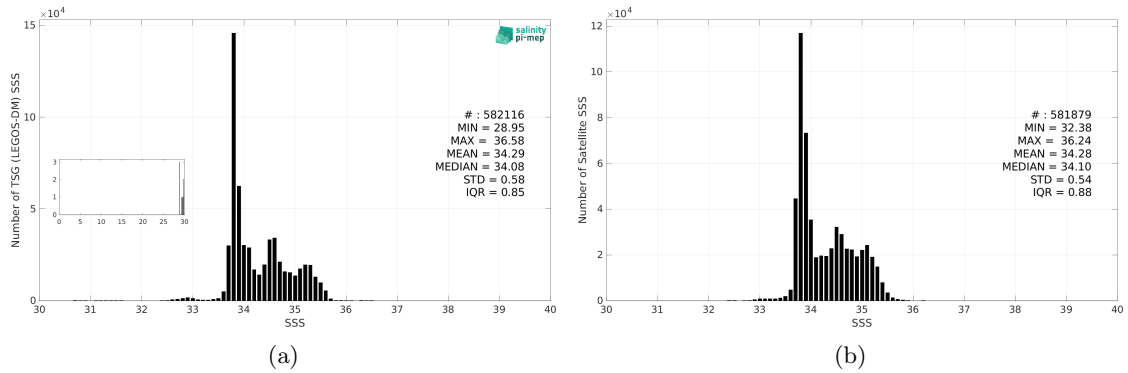
Figure 3: Histograms of SSS from TSG (LEGOS-DM) (a) and SMOS SSS L4 v1 - Daily (CMEMS-CNR) (b) considering all match-up pairs per bins of 0.1 over the Roaring Forties and Furious Fifties Pi-MEP region and for the full satellite product period.
