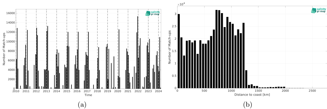
Figure 2: Number of match-ups between TSG (LEGOS-DM) and SMOS SSS L4 v1 - Daily (CMEMS-CNR) SSS as a function of time (a) and as function of the distance to coast (b) over the Roaring Forties and Furious Fifties Pi-MEP region and for the full satellite product period.
