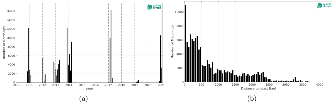
Figure 2: Number of match-ups between TSG (GOSUD-Sailing-ship) and SMOS SSS L4 v1 - Daily (CMEMS-CNR) SSS as a function of time (a) and as function of the distance to coast (b) over the Roaring Forties and Furious Fifties Pi-MEP region and for the full satellite product period.
