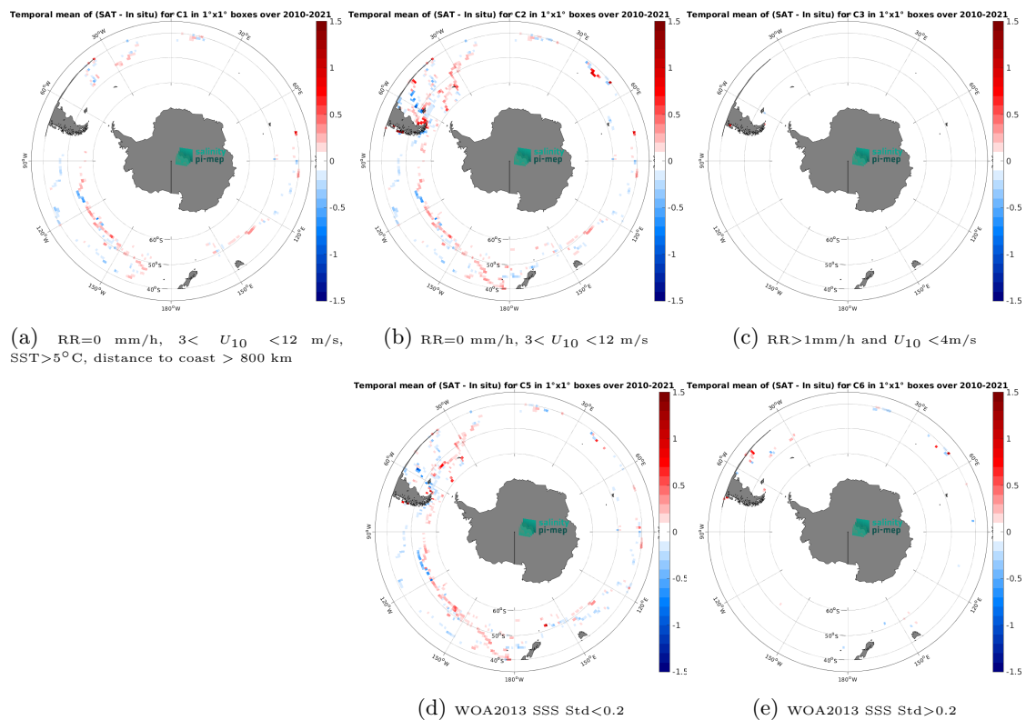
Figure 14: Temporal mean gridded over spatial boxes of size 1^\circ \times 1^\circ of \Delta SSS (SMOS SSS L4 v1 - Daily (CMEMS-CNR) - TSG (GOSUD-Sailing-ship)) for 5 different subdatasets corresponding to: RR=0 mm/h, 3 < U_{10} < 12 m/s, SST > 5^\circ\text{C} , distance to coast > 800 km (a), RR=0 mm/h, 3 < U_{10} < 12 m/s (b), RR > 1 mm/h and U_{10} < 4 m/s (c), WOA2013 SSS Std < 0.2 (d), WOA2013 SSS Std > 0.2 (e).
