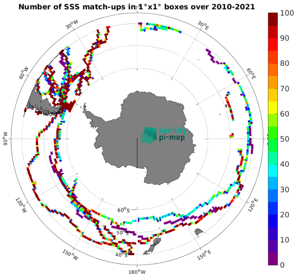
Figure 5: Number of SSS match-ups between TSG (GOSUD-Sailing-ship) SSS and the SMOS SSS L4 v1 - Daily (CMEMS-CNR) SSS product for the Roaring Forties and Furious Fifties Pi-MEP region over 1^\circ \times 1^\circ boxes and for the full satellite product period.
