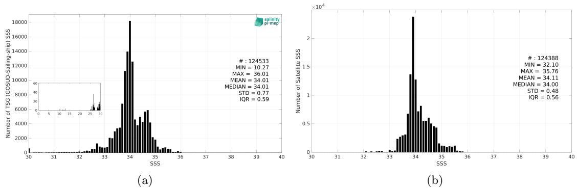
Figure 3: Histograms of SSS from TSG (GOSUD-Sailing-ship) (a) and SMOS SSS L4 v1 - Daily (CMEMS-CNR) (b) considering all match-up pairs per bins of 0.1 over the Roaring Forties and Furious Fifties Pi-MEP region and for the full satellite product period.
