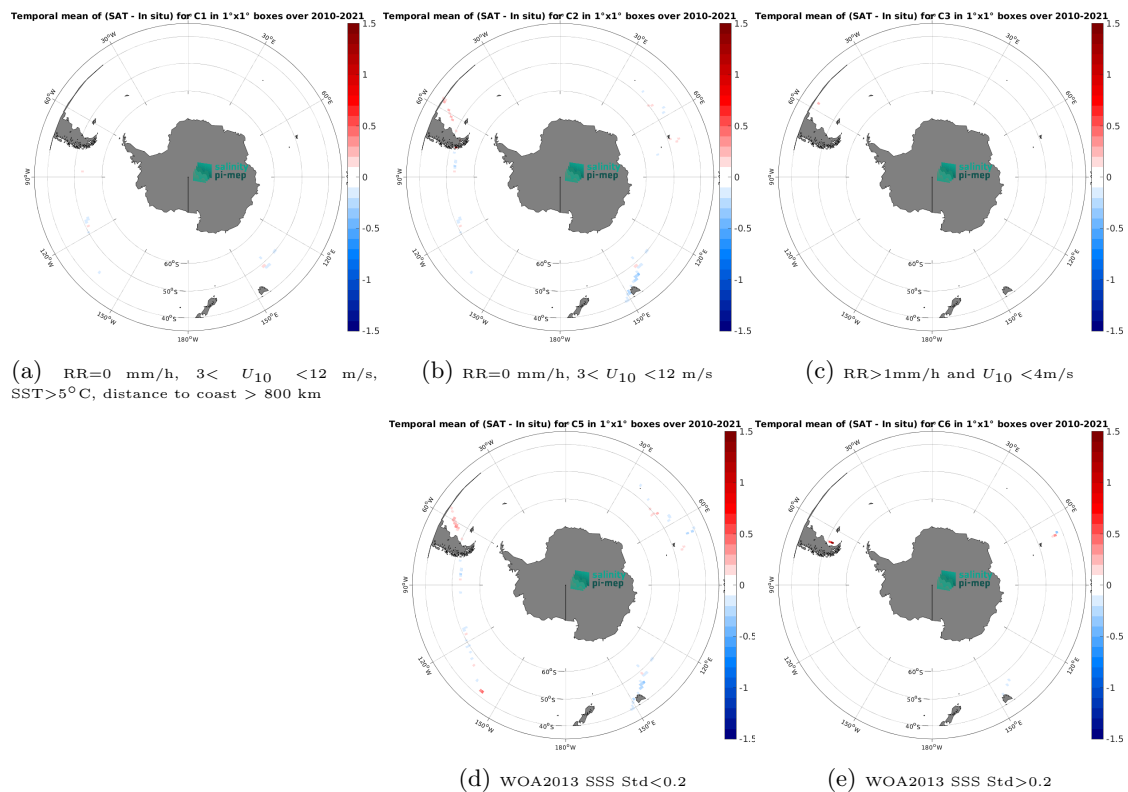
Figure 14: Temporal mean gridded over spatial boxes of size 1^\circ \times 1^\circ of \Delta\text{SSS} (SMOS SSS L4 v1 - Daily (CMEMS-CNR) - TSG (GOSUD-Research-vessel)) for 5 different subdatasets corresponding to:RR=0 mm/h, 3 < U_{10} < 12 m/s, SST>5°C, distance to coast > 800 km (a), RR=0 mm/h, 3 < U_{10} < 12 m/s (b), RR>1mm/h and U_{10} < 4 m/s (c), WOA2013 SSS Std<0.2 (d), WOA2013 SSS Std>0.2 (e).
