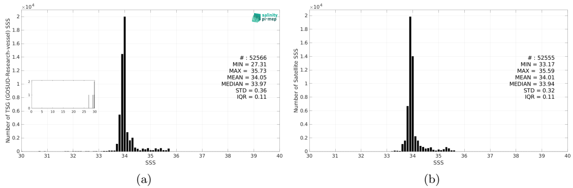
Figure 3: Histograms of SSS from TSG (GOSUD-Research-vessel) (a) and SMOS SSS L4 v1 - Daily (CMEMS-CNR) (b) considering all match-up pairs per bins of 0.1 over the Roaring Forties and Furious Fifties Pi-MEP region and for the full satellite product period.
