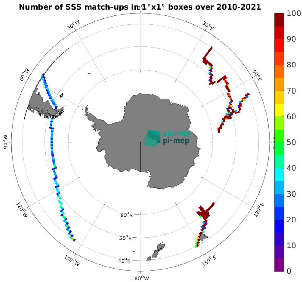
Figure 5: Number of SSS match-ups between TSG (GOSUD-Research-vessel) SSS and the SMOS SSS L4 v1 - Daily (CMEMS-CNR) SSS product for the Roaring Forties and Furious Fifties Pi-MEP region over 1^\circ \times 1^\circ boxes and for the full satellite product period.
