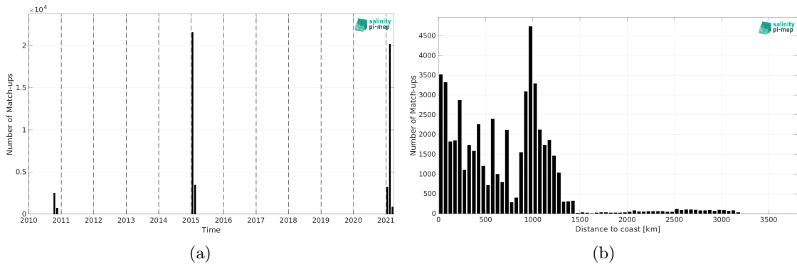
Figure 2: Number of match-ups between TSG (GOSUD-Research-vessel) and SMOS SSS L4 v1 - Daily (CMEMS-CNR) SSS as a function of time (a) and as function of the distance to coast (b) over the Roaring Forties and Furious Fifties Pi-MEP region and for the full satellite product period.
