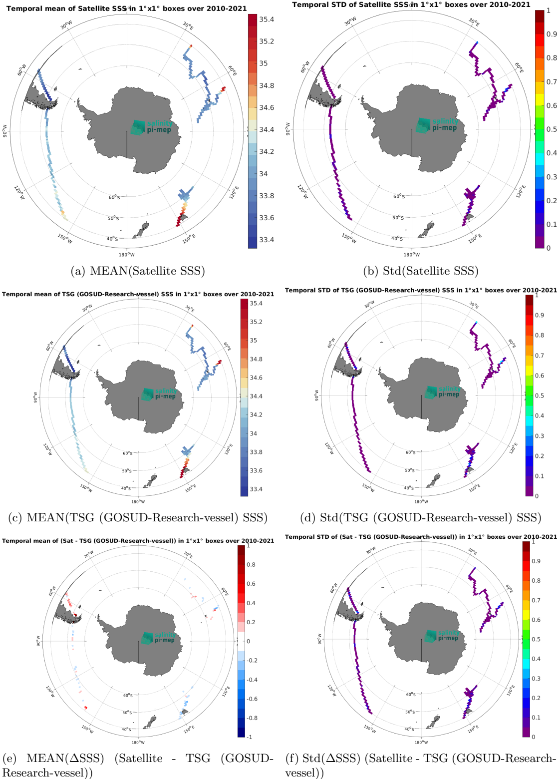
Figure 7: Temporal mean (left) and Std (right) of SSS from SMOS SSS L4 v1 - Daily (CMEMS-CNR) (top), TSG (GOSUD-Research-vessel) (middle), and of \Delta SSS (Satellite - TSG (GOSUD-Research-vessel)). Only match-up pairs are used to generate these maps.
