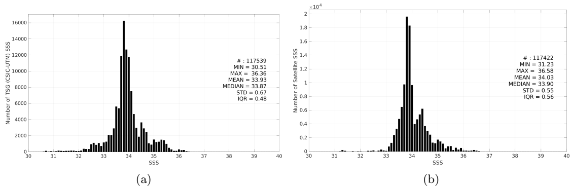
Figure 3: Histograms of SSS from TSG (CSIC-UTM) (a) and SMOS SSS L4 v1 - Daily (CMEMS-CNR) (b) considering all match-up pairs per bins of 0.1 over the Roaring Forties and Furious Fifties Pi-MEP region and for the full satellite product period.
