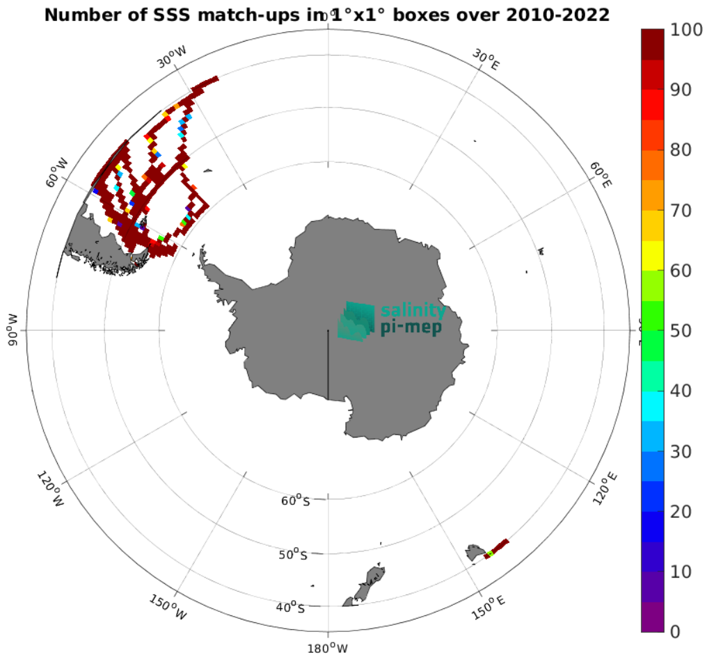
Figure 5: Number of SSS match-ups between TSG (CSIC-UTM) SSS and the SMOS SSS L4 v1 - Daily (CMEMS-CNR) SSS product for the Roaring Forties and Furious Fifties Pi-MEP region over 1^\circ \times 1^\circ boxes and for the full satellite product period.
