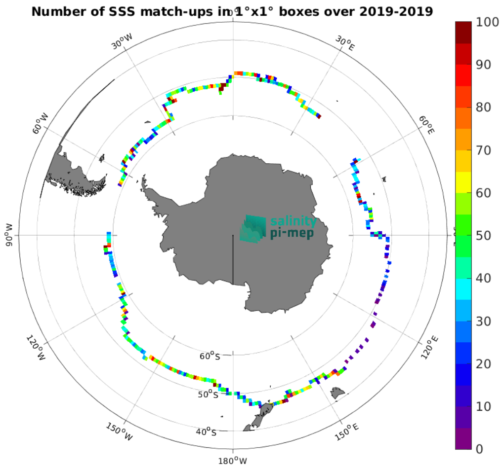
Figure 5: Number of SSS match-ups between Saildrone SSS and the SMOS SSS L4 v1 - Daily (CMEMS-CNR) SSS product for the Roaring Forties and Furious Fifties Pi-MEP region over 1^\circ \times 1^\circ boxes and for the full satellite product period.
