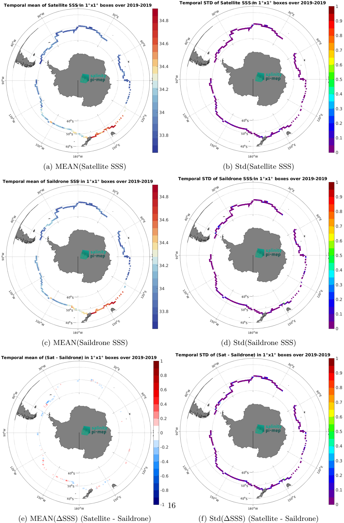
Figure 7: Temporal mean (left) and Std (right) of SSS from SMOS SSS L4 v1 - Daily (CMEMS-CNR) (top), Saildrone (middle), and of \Delta SSS (Satellite - Saildrone). Only match-up pairs are used to generate these maps.
