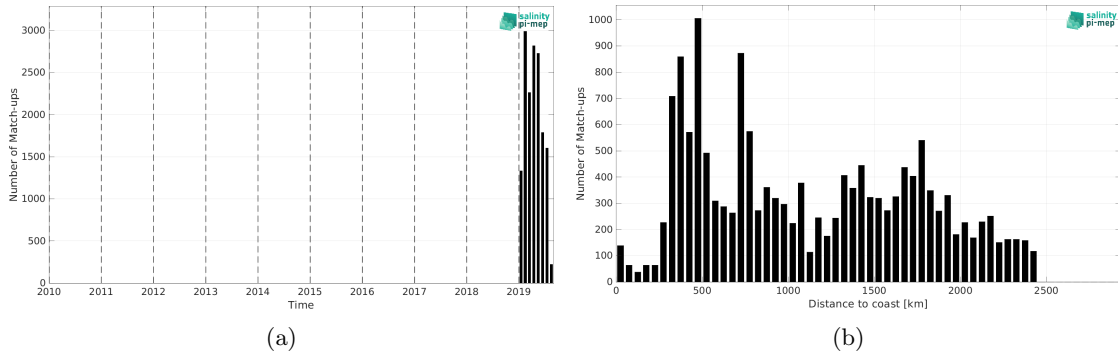
Figure 2: Number of match-ups between Saildrone and SMOS SSS L4 v1 - Daily (CMEMS-CNR) SSS as a function of time (a) and as function of the distance to coast (b) over the Roaring Forties and Furious Fifties Pi-MEP region and for the full satellite product period.
