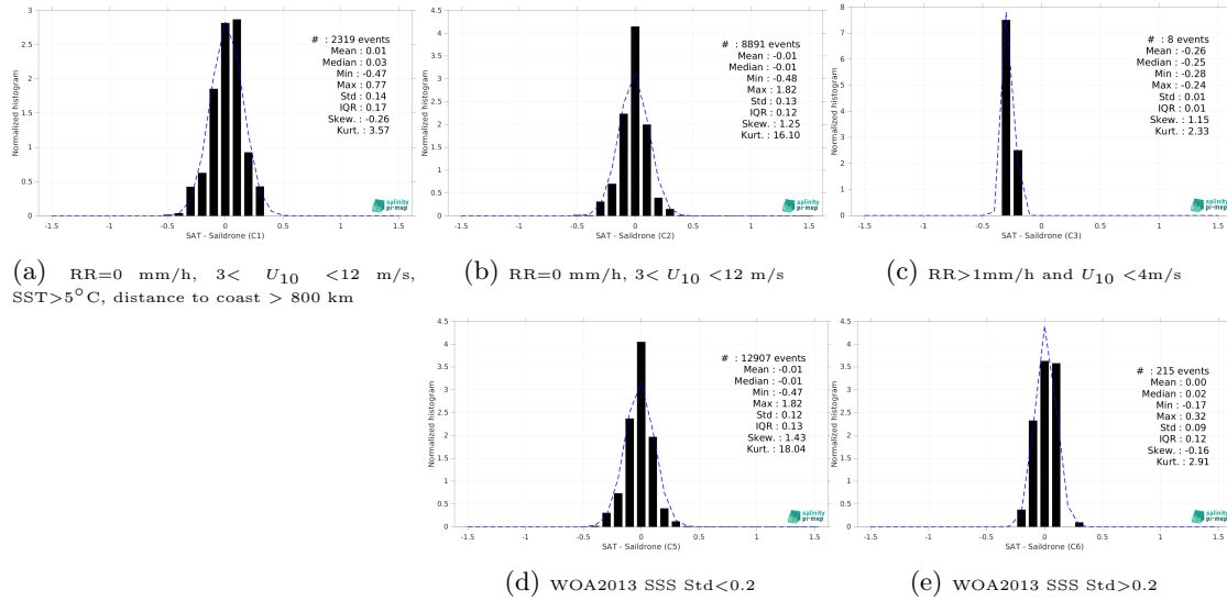
Figure 15: Normalized histogram of \Delta\text{SSS} (SMOS SSS L4 v1 - Daily (CMEMS-CNR) - Saldrone) for 5 different subdatasets corresponding to: RR=0 mm/h, 3 < U_{10} < 12 m/s, SST>5°C, distance to coast > 800 km (a), RR=0 mm/h, 3 < U_{10} < 12 m/s (b), RR>1mm/h and U_{10} < 4 m/s (c), WOA2013 SSS Std<0.2 (d), WOA2013 SSS Std>0.2 (e).
