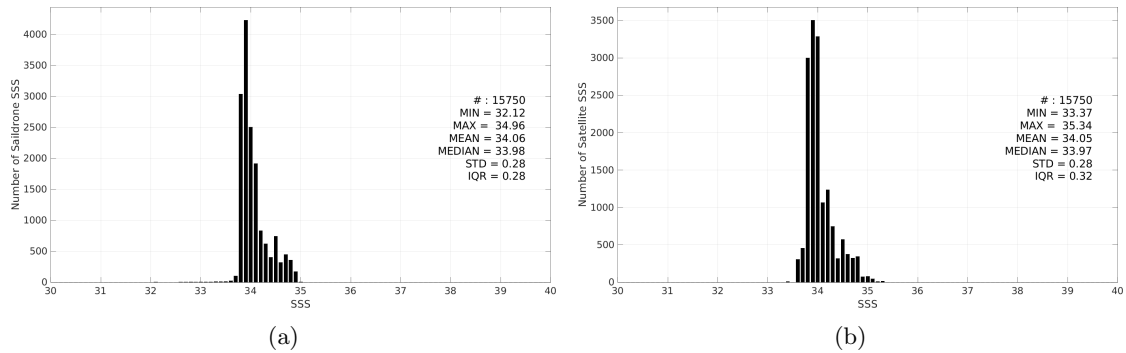
Figure 3: Histograms of SSS from Saildrone (a) and SMOS SSS L4 v1 - Daily (CMEMS-CNR) (b) considering all match-up pairs per bins of 0.1 over the Roaring Forties and Furious Fifties Pi-MEP region and for the full satellite product period.
