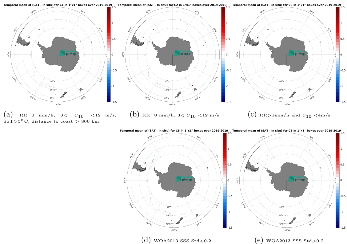
Figure 14: Temporal mean gridded over spatial boxes of size 1^\circ \times 1^\circ of \Delta\text{SSS} (SMOS SSS L4 v1 - Daily (CMEMS-CNR) - Sairdrone) for 5 different subdatasets corresponding to:RR=0 mm/h, 3 < U_{10} < 12 m/s, SST>5°C, distance to coast > 800 km (a), RR=0 mm/h, 3 < U_{10} < 12 m/s (b), RR>1mm/h and U_{10} < 4 m/s (c), WOA2013 SSS Std<0.2 (d), WOA2013 SSS Std>0.2 (e).
