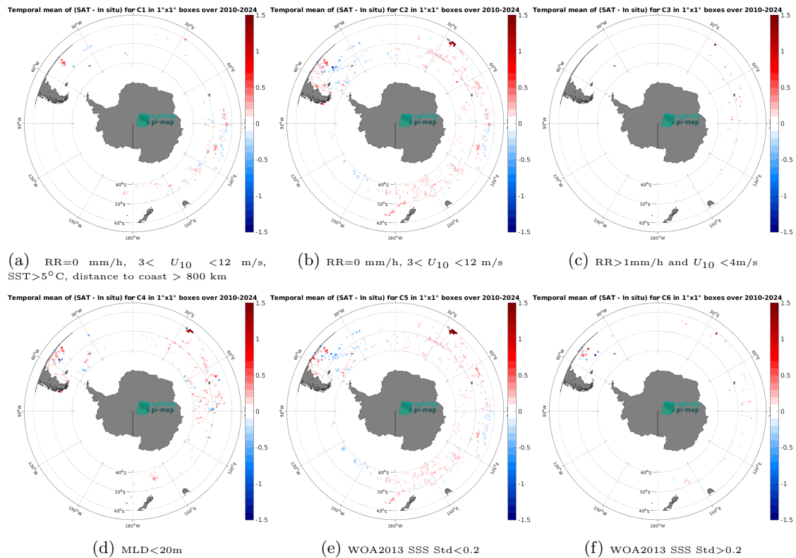
Figure 14: Temporal mean gridded over spatial boxes of size 1^\circ \times 1^\circ of \Delta SSS (SMOS SSS L4 v1 - Daily (CMEMS-CNR) - Marine mammals) for 6 different subdatasets corresponding to:RR=0 mm/h, 3 < U_{10} < 12 m/s, SST>5°C, distance to coast > 800 km (a), RR=0 mm/h, 3 < U_{10} < 12 m/s (b), RR>1mm/h and U_{10} < 4 m/s (c),MLD<20m (d),WOA2013 SSS Std<0.2 (e),WOA2013 SSS Std>0.2 (f).
