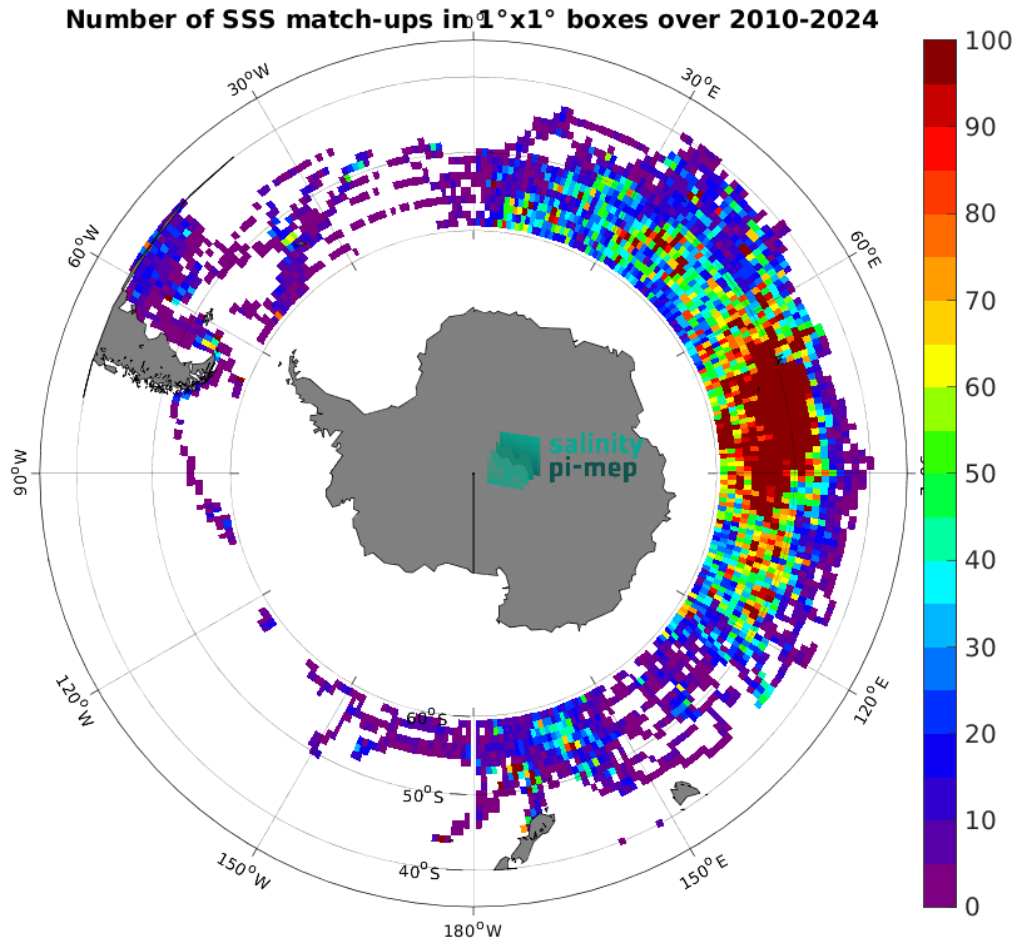
Figure 5: Number of SSS match-ups between Marine mammals SSS and the SMOS SSS L4 v1 - Daily (CMEMS-CNR) SSS product for the Roaring Forties and Furious Fifties Pi-MEP region over 1^\circ \times 1^\circ boxes and for the full satellite product period.
