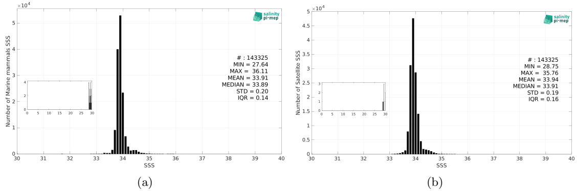
Figure 3: Histograms of SSS from Marine mammals (a) and SMOS SSS L4 v1 - Daily (CMEMS-CNR) (b) considering all match-up pairs per bins of 0.1 over the Roaring Forties and Furious Fifties Pi-MEP region and for the full satellite product period.
