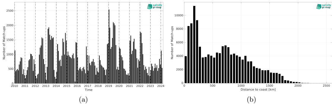
Figure 2: Number of match-ups between Marine mammals and SMOS SSS L4 v1 - Daily (CMEMS-CNR) SSS as a function of time (a) and as function of the distance to coast (b) over the Roaring Forties and Furious Fifties Pi-MEP region and for the full satellite product period.
