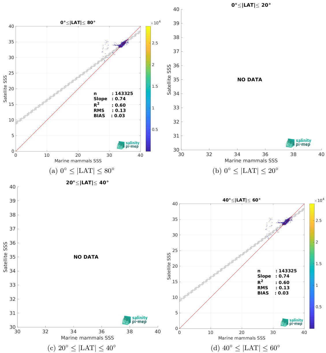
Figure 10: Contour maps of the concentration of SMOS SSS L4 v1 - Daily (CMEMS-CNR) SSS (y-axis) versus Marine mammals SSS (x-axis) at match-up pairs for different latitude bands. For each plot, the red line shows x=y . The black thin and dashed lines indicate a linear fit through the data cloud and the \pm 95\% confidence levels, respectively. The number match-up pairs n , the slope and R^2 coefficient of the linear fit, the root mean square (RMS) and the mean bias between satellite and in situ data are indicated for each latitude band in each plots.
