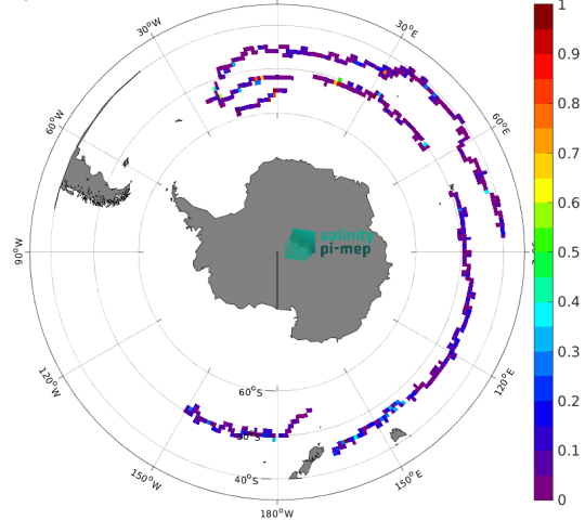
(e) MEAN( \Delta SSS) (Satellite - Surface drifters)
