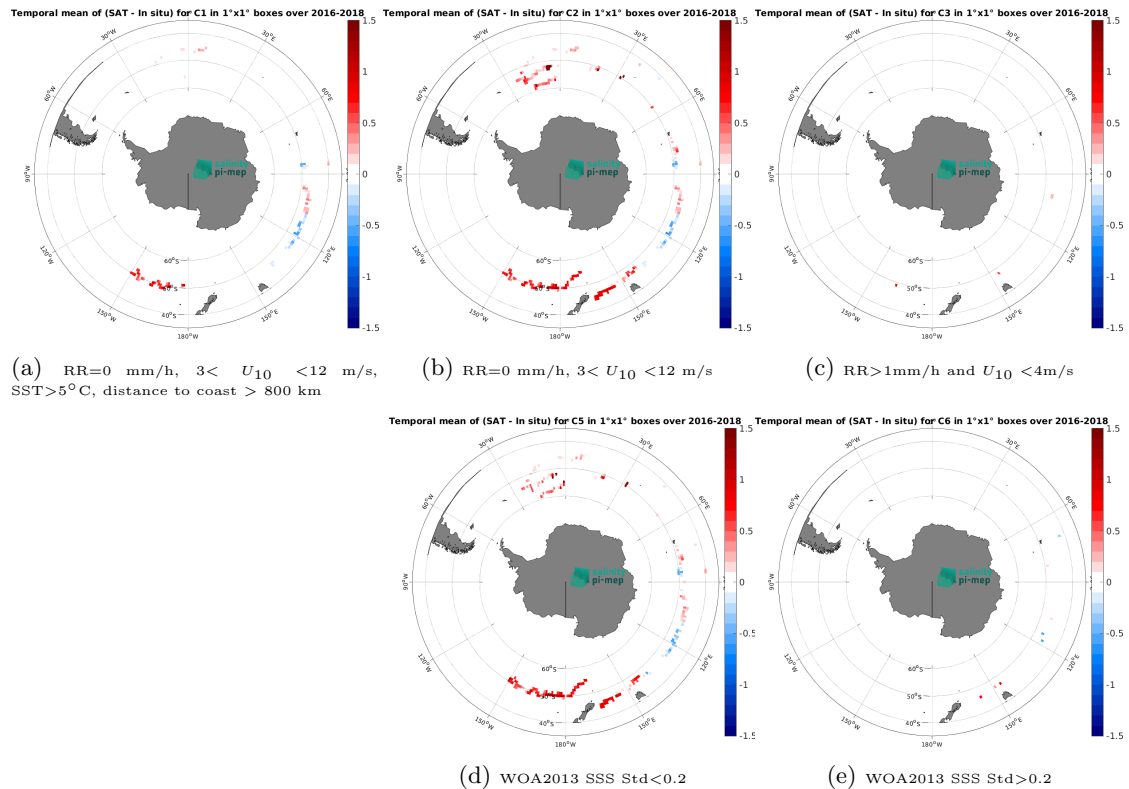
Figure 13: Temporal mean gridded over spatial boxes of size 1^\circ \times 1^\circ of \Delta SSS (SMOS SSS L4 v1 - Daily (CMEMS-CNR) - Surface drifters) for 5 different subdatasets corresponding to:RR=0 mm/h, 3 < U_{10} < 12 m/s, SST >5^\circ\text{C} , distance to coast > 800 km (a), RR=0 mm/h, 3 < U_{10} < 12 m/s (b), RR >1 mm/h and U_{10} < 4 m/s (c), WOA2013 SSS Std <0.2 (d), WOA2013 SSS Std >0.2 (e).
