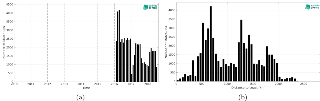
Figure 2: Number of match-ups between Surface drifters and SMOS SSS L4 v1 - Daily (CMEMS-CNR) SSS as a function of time (a) and as function of the distance to coast (b) over the Roaring Forties and Furious Fifties Pi-MEP region and for the full satellite product period.
