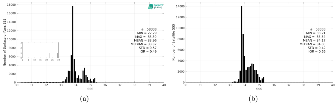
Figure 3: Histograms of SSS from Surface drifters (a) and SMOS SSS L4 v1 - Daily (CMEMS-CNR) (b) considering all match-up pairs per bins of 0.1 over the Roaring Forties and Furious Fifties Pi-MEP region and for the full satellite product period.
