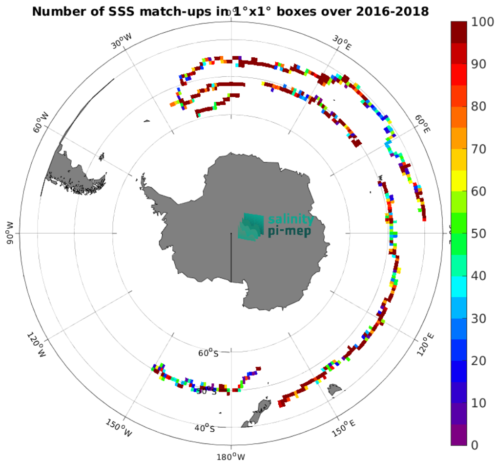
Figure 4: Number of SSS match-ups between Surface drifters SSS and the SMOS SSS L4 v1 - Daily (CMEMS-CNR) SSS product for the Roaring Forties and Furious Fifties Pi-MEP region over 1^\circ \times 1^\circ boxes and for the full satellite product period.
