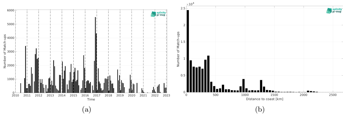
Figure 2: Number of match-ups between TSG (SAMOS) and SMOS SSS L4 OI v346 - Weekly (CMEMS-CATDS-LOPS) SSS as a function of time (a) and as function of the distance to coast (b) over the Roaring Forties and Furious Fifties Pi-MEP region and for the full satellite product period.
