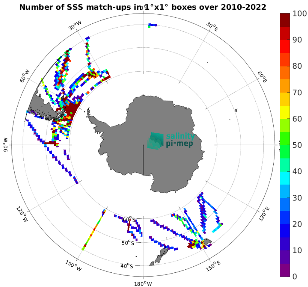
Figure 5: Number of SSS match-ups between TSG (SAMOS) SSS and the SMOS SSS L4 OI v346 - Weekly (CMEMS-CATDS-LOPS) SSS product for the Roaring Forties and Furious Fifties Pi-MEP region over 1^\circ \times 1^\circ boxes and for the full satellite product period.
