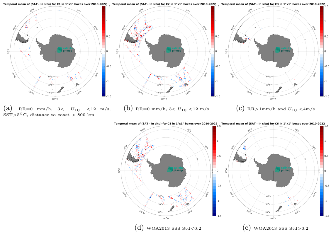
Figure 14: Temporal mean gridded over spatial boxes of size 1^\circ \times 1^\circ of \Delta\text{SSS} (SMOS SSS L4 OI v346 - Weekly (CMEMS-CATDS-LOPS) - TSG (SAMOS)) for 5 different subdatasets corresponding to:RR=0 mm/h, 3 < U_{10} < 12 m/s, SST > 5°C, distance to coast > 800 km (a), RR=0 mm/h, 3 < U_{10} < 12 m/s (b), RR > 1mm/h and U_{10} < 4 m/s (c), WOA2013 SSS Std < 0.2 (d), WOA2013 SSS Std > 0.2 (e).
