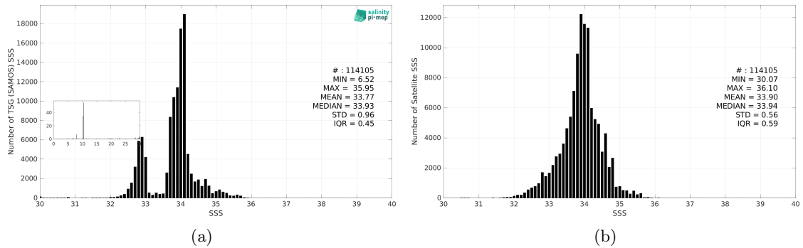
Figure 3: Histograms of SSS from TSG (SAMOS) (a) and SMOS SSS L4 OI v346 - Weekly (CMEMS-CATDS-LOPS) (b) considering all match-up pairs per bins of 0.1 over the Roaring Forties and Furious Fifties Pi-MEP region and for the full satellite product period.
