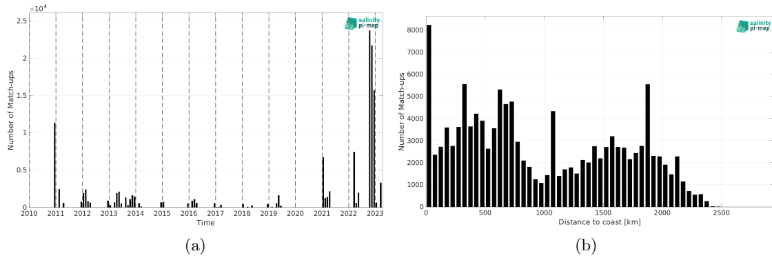
Figure 2: Number of match-ups between TSG (Polarstern) and SMOS SSS L4 OI v346 - Weekly (CMEMS-CATDS-LOPS) SSS as a function of time (a) and as function of the distance to coast (b) over the Roaring Forties and Furious Fifties Pi-MEP region and for the full satellite product period.
