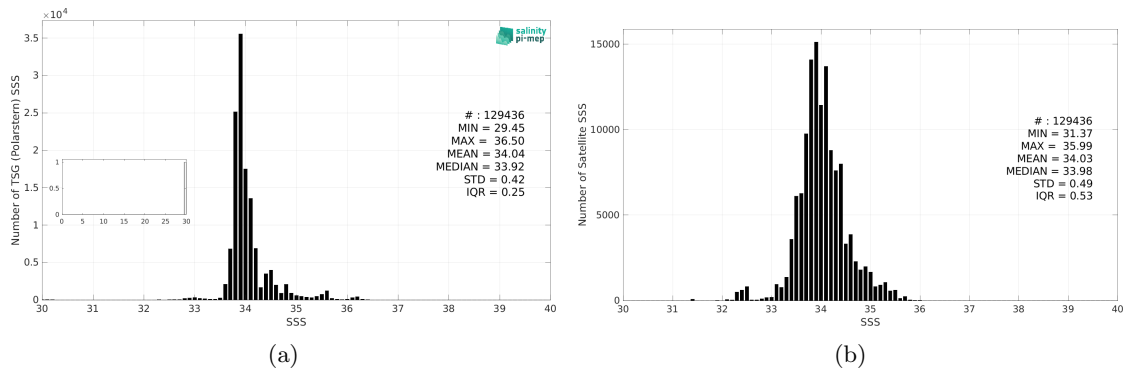
Figure 3: Histograms of SSS from TSG (Polarstern) (a) and SMOS SSS L4 OI v346 - Weekly (CMEMS-CATDS-LOPS) (b) considering all match-up pairs per bins of 0.1 over the Roaring Forties and Furious Fifties Pi-MEP region and for the full satellite product period.
