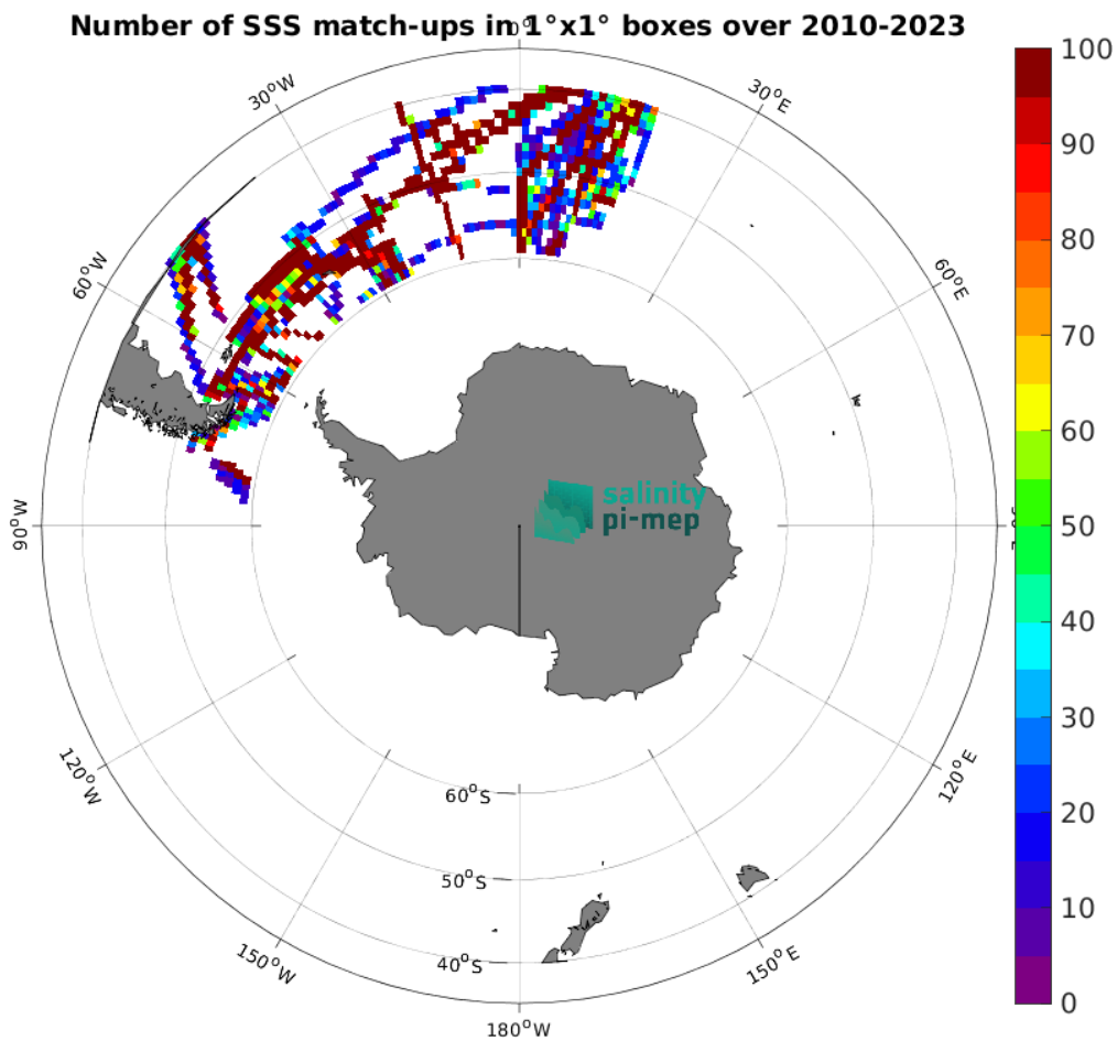
Figure 5: Number of SSS match-ups between TSG (Polarstern) SSS and the SMOS SSS L4 OI v346 - Weekly (CMEMS-CATDS-LOPS) SSS product for the Roaring Forties and Furious Fifties Pi-MEP region over 1^\circ \times 1^\circ boxes and for the full satellite product period.
