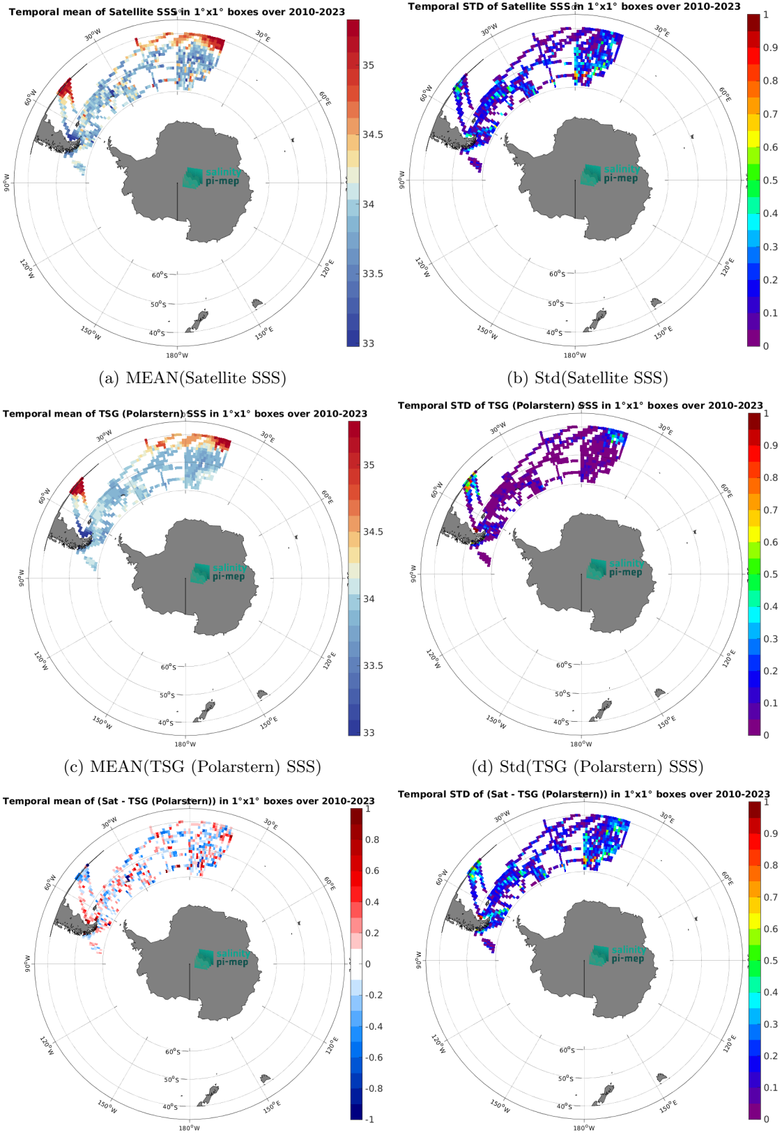
(a) MEAN(Satellite SSS) (b) Std(Satellite SSS) (c) MEAN(TSG (Polarstern) SSS) (d) Std(TSG (Polarstern) SSS) (e) MEAN( \Delta SSS) (Satellite - TSG (Polarstern)) (f) Std( \Delta SSS) (Satellite - TSG (Polarstern)) Figure 7: Temporal mean (left) and Std (right) of SSS from SMOS SSS L4 OI v346 - Weekly (CMEMS-CATDS-LOPS) (top), TSG (Polarstern) (middle), and of \Delta SSS (Satellite - TSG (Polarstern)). Only match-up pairs are used to generate these maps.
