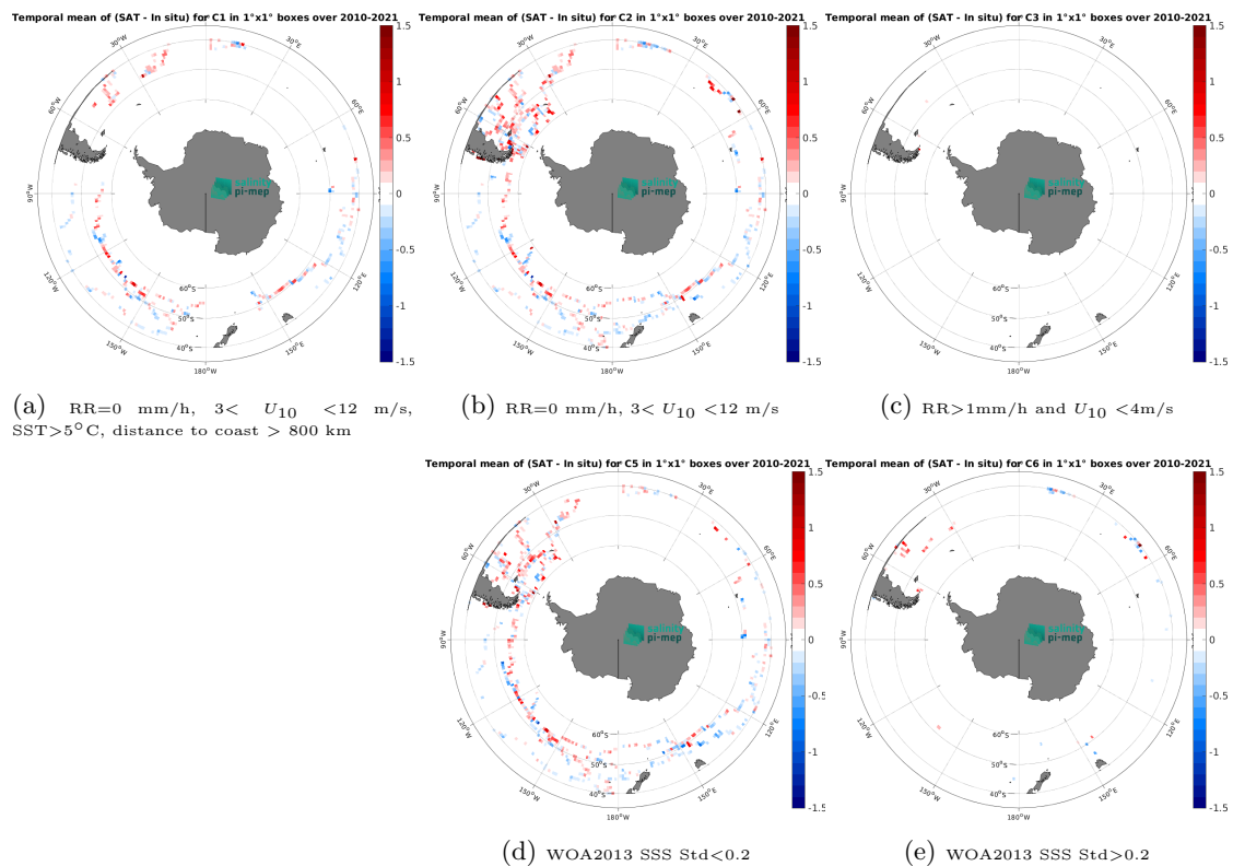
Figure 14: Temporal mean gridded over spatial boxes of size 1^\circ \times 1^\circ of \Delta\text{SSS} (SMOS SSS L4 OI v346 - Weekly (CMEMS-CATDS-LOPS) - TSG (GOSUD-Sailing-ship)) for 5 different sub-datasets corresponding to:RR=0 mm/h, 3 < U_{10} < 12 m/s, SST>5°C, distance to coast > 800 km (a), RR=0 mm/h, 3 < U_{10} < 12 m/s (b), RR>1mm/h and U_{10} < 4 m/s (c), WOA2013 SSS Std<0.2 (d), WOA2013 SSS Std>0.2 (e).
