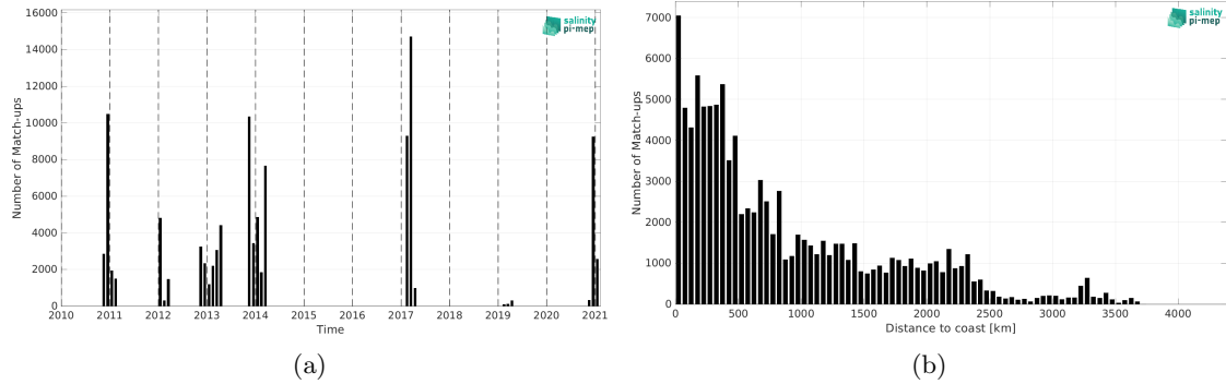
Figure 2: Number of match-ups between TSG (GOSUD-Sailing-ship) and SMOS SSS L4 OI v346 - Weekly (CMEMS-CATDS-LOPS) SSS as a function of time (a) and as function of the distance to coast (b) over the Roaring Forties and Furious Fifties Pi-MEP region and for the full satellite product period.
