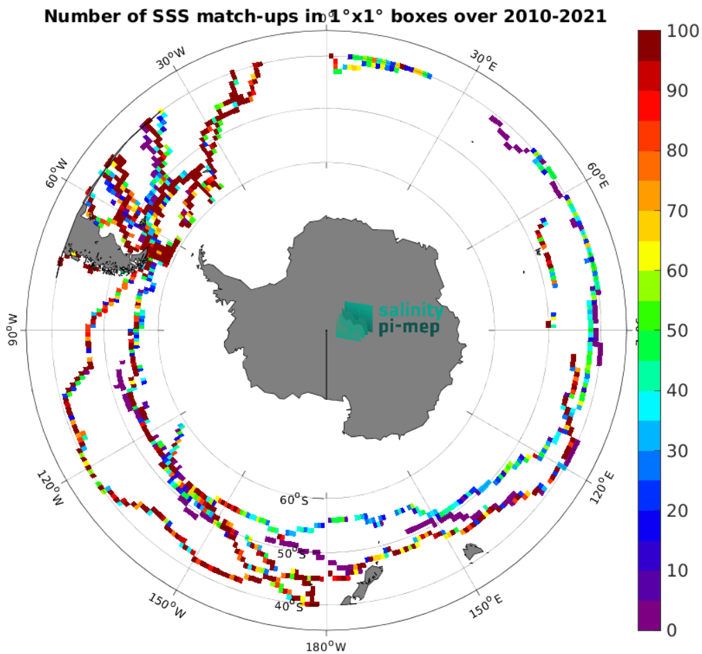
Figure 5: Number of SSS match-ups between TSG (GOSUD-Sailing-ship) SSS and the SMOS SSS L4 OI v346 - Weekly (CMEMS-CATDS-LOPS) SSS product for the Roaring Forties and Furious Fifties Pi-MEP region over 1^\circ \times 1^\circ boxes and for the full satellite product period.
