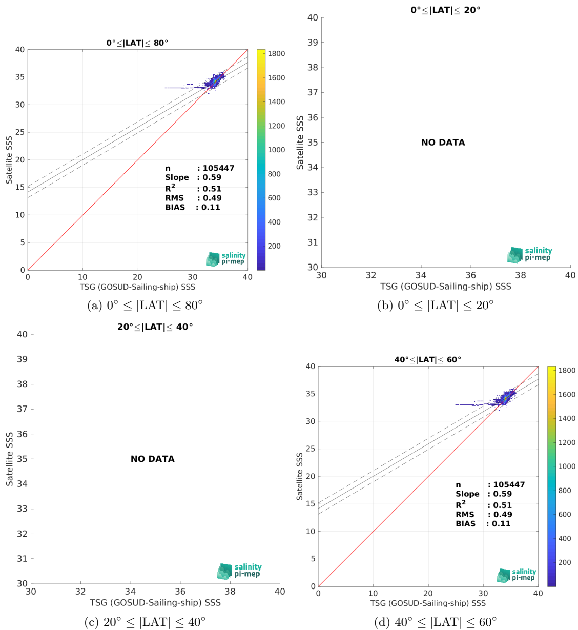
Figure 10: Contour maps of the concentration of SMOS SSS L4 OI v346 - Weekly (CMEMS-CATDS-LOPS) SSS (y-axis) versus TSG (GOSUD-Sailing-ship) SSS (x-axis) at match-up pairs for different latitude bands. For each plot, the red line shows x=y . The black thin and dashed lines indicate a linear fit through the data cloud and the \pm 95\% confidence levels, respectively. The number match-up pairs n , the slope and R^2 coefficient of the linear fit, the root mean square (RMS) and the mean bias between satellite and in situ data are indicated for each latitude band in each plots.
