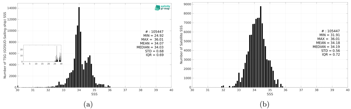
Figure 3: Histograms of SSS from TSG (GOSUD-Sailing-ship) (a) and SMOS SSS L4 OI v346 - Weekly (CMEMS-CATDS-LOPS) (b) considering all match-up pairs per bins of 0.1 over the Roaring Forties and Furious Fifties Pi-MEP region and for the full satellite product period.
