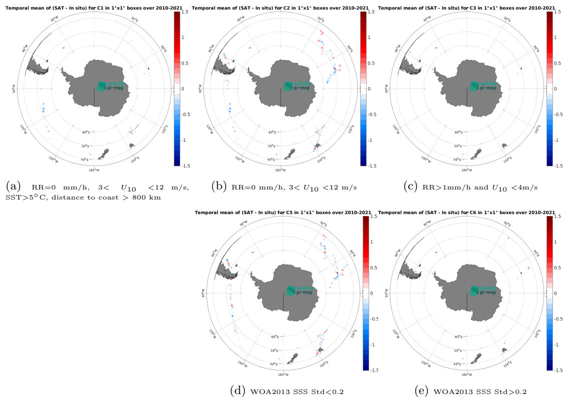
Figure 14: Temporal mean gridded over spatial boxes of size 1^\circ \times 1^\circ of \Delta\text{SSS} (SMOS SSS L4 OI v346 - Weekly (CMEMS-CATDS-LOPS) - TSG (GOSUD-Research-vessel)) for 5 different subdatasets corresponding to:RR=0 mm/h, 3 < U_{10} < 12 m/s, SST>5°C, distance to coast > 800 km (a), RR=0 mm/h, 3 < U_{10} < 12 m/s (b), RR>1mm/h and U_{10} < 4 m/s (c), WOA2013 SSS Std<0.2 (d), WOA2013 SSS Std>0.2 (e).
