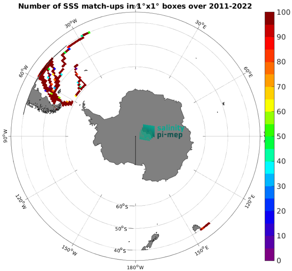
Figure 5: Number of SSS match-ups between TSG (CSIC-UTM) SSS and the SMOS SSS L4 OI v346 - Weekly (CMEMS-CATDS-LOPS) SSS product for the Roaring Forties and Furious Fifties Pi-MEP region over 1^\circ \times 1^\circ boxes and for the full satellite product period.
