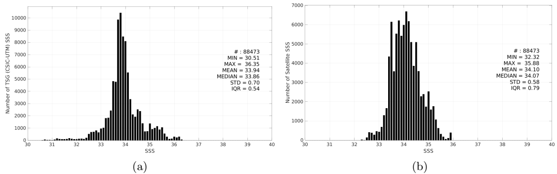
Figure 3: Histograms of SSS from TSG (CSIC-UTM) (a) and SMOS SSS L4 OI v346 - Weekly (CMEMS-CATDS-LOPS) (b) considering all match-up pairs per bins of 0.1 over the Roaring Forties and Furious Fifties Pi-MEP region and for the full satellite product period.
