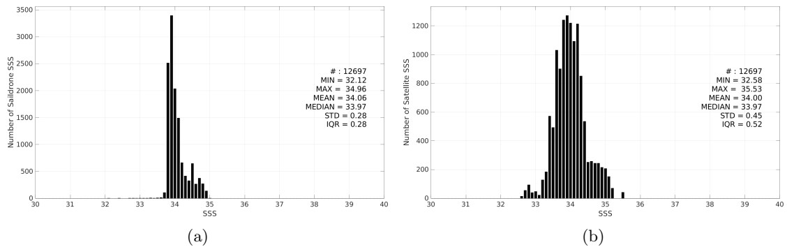
Figure 3: Histograms of SSS from Saildrone (a) and SMOS SSS L4 OI v346 - Weekly (CMEMS-CATDS-LOPS) (b) considering all match-up pairs per bins of 0.1 over the Roaring Forties and Furious Fifties Pi-MEP region and for the full satellite product period.
