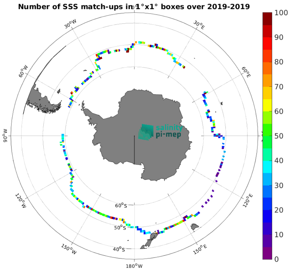
Figure 5: Number of SSS match-ups between Saildrone SSS and the SMOS SSS L4 OI v346 - Weekly (CMEMS-CATDS-LOPS) SSS product for the Roaring Forties and Furious Fifties Pi-MEP region over 1^\circ \times 1^\circ boxes and for the full satellite product period.
