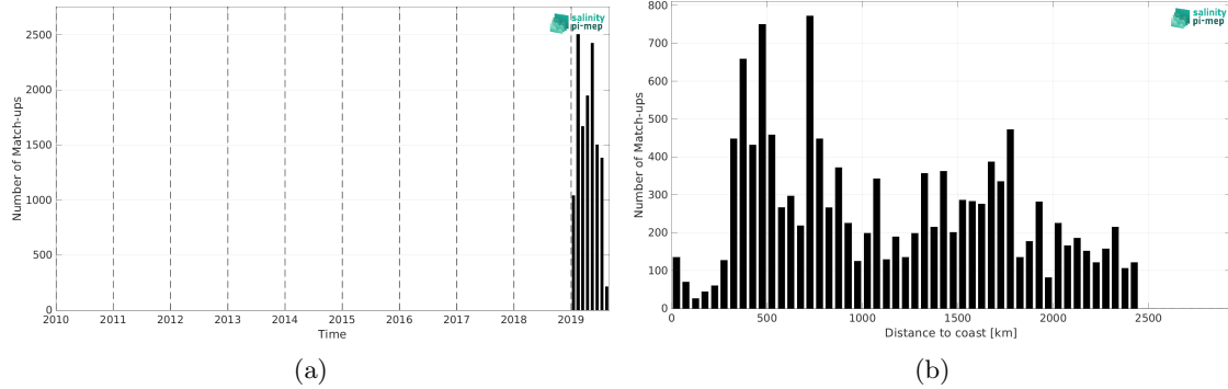
Figure 2: Number of match-ups between Saildrone and SMOS SSS L4 OI v346 - Weekly (CMEMS-CATDS-LOPS) SSS as a function of time (a) and as function of the distance to coast (b) over the Roaring Forties and Furious Fifties Pi-MEP region and for the full satellite product period.
