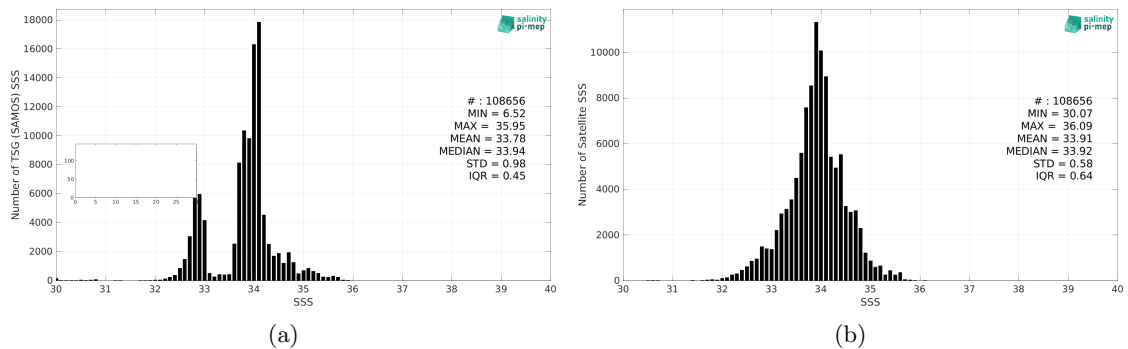
Figure 2: Histograms of SSS from TSG (SAMOS) (a) and SMOS SSS L4 OI v342 - Weekly (CMEMS-CATDS-LOPS) (b) considering all match-up pairs per bins of 0.1 over the Roaring Forties and Furious Fifties Pi-MEP region and for the full satellite product period.
