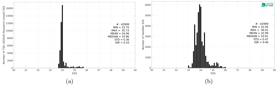
Figure 2: Histograms of SSS from TSG (GOSUD-Research-vessel) (a) and SMOS SSS L4 OI v342 - Weekly (CMEMS-CATDS-LOPS) (b) considering all match-up pairs per bins of 0.1 over the Roaring Forties and Furious Fifties Pi-MEP region and for the full satellite product period.
