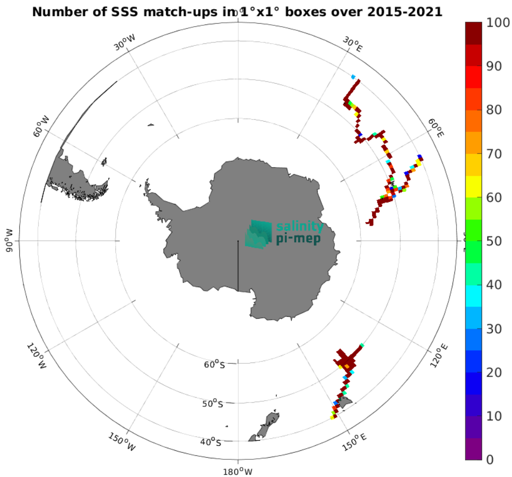
Figure 4: Number of SSS match-ups between TSG (GOSUD-Research-vessel) SSS and the SMOS SSS L4 OI v342 - Weekly (CMEMS-CATDS-LOPS) SSS product for the Roaring Forties and Furious Fifties Pi-MEP region over 1^\circ \times 1^\circ boxes and for the full satellite product period.
