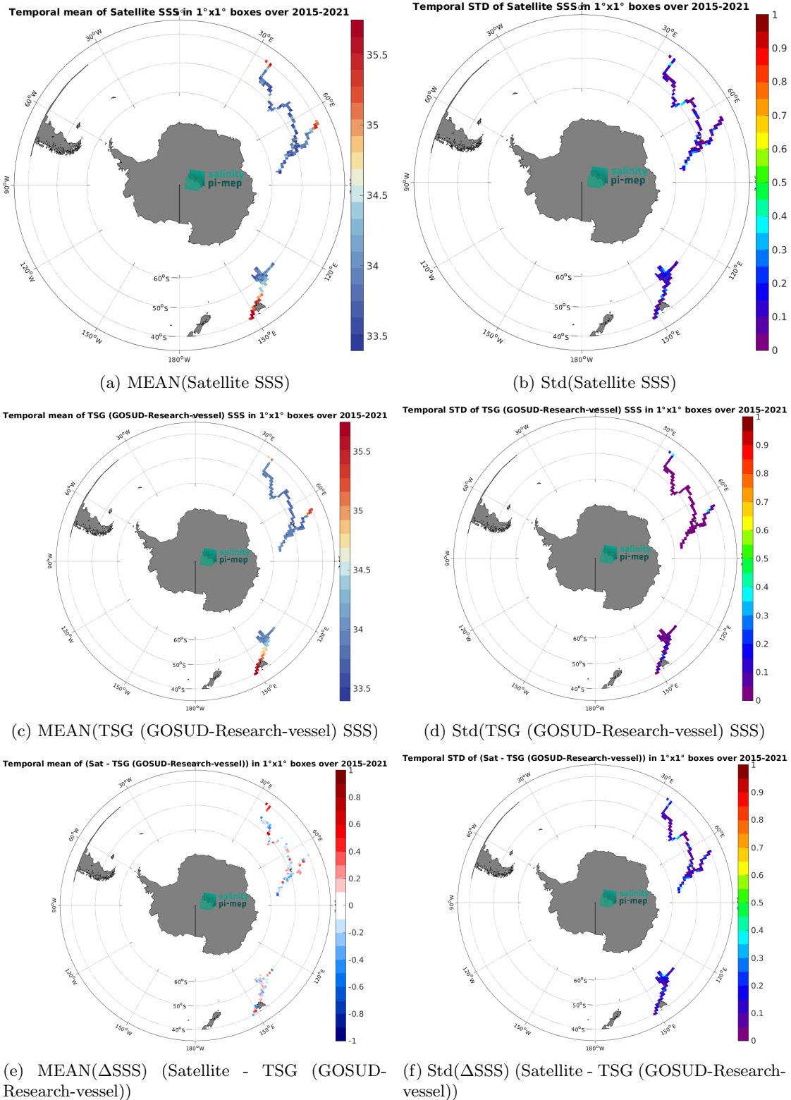
Figure 6: Temporal mean (left) and Std (right) of SSS from SMOS SSS L4 OI v342 - Weekly (CMEMS-CATDS-LOPS) (top), TSG (GOSUD-Research-vessel) (middle), and of \Delta SSS (Satellite - TSG (GOSUD-Research-vessel)). Only 17 up-ch pairs are used to generate these maps.
