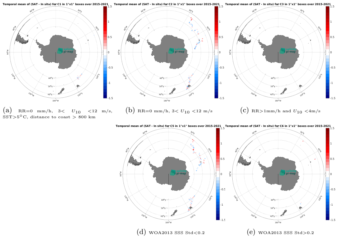
Figure 12: Temporal mean gridded over spatial boxes of size 1^\circ \times 1^\circ of \Delta SSS (SMOS SSS L4 OI v342 - Weekly (CMEMS-CATDS-LOPS) - TSG (GOSUD-Research-vessel)) for 5 different subdatasets corresponding to:RR=0 mm/h, 3 < U_{10} < 12 m/s, SST>5°C, distance to coast > 800 km (a), RR=0 mm/h, 3 < U_{10} < 12 m/s (b), RR>1mm/h and U_{10} < 4 m/s (c), WOA2013 SSS Std<0.2 (d), WOA2013 SSS Std>0.2 (e).
