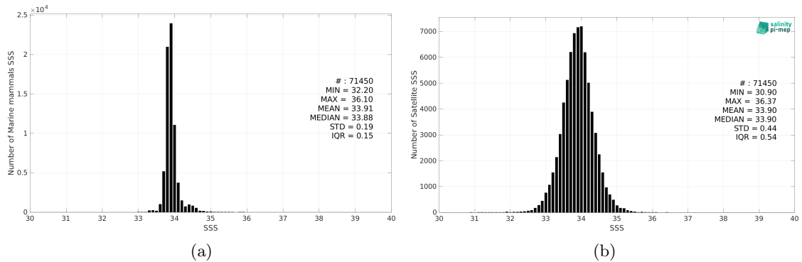
Figure 2: Histograms of SSS from Marine mammals (a) and SMOS SSS L4 OI v342 - Weekly (CMEMS-CATDS-LOPS) (b) considering all match-up pairs per bins of 0.1 over the Roaring Forties and Furious Fifties Pi-MEP region and for the full satellite product period.
