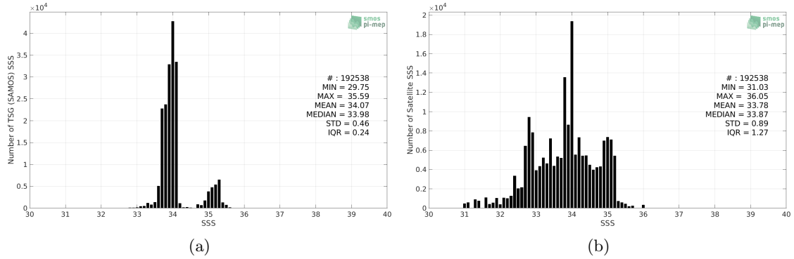
Figure 2: Histograms of SSS from TSG (SAMOS) (a) and SMOS L4 v2 Weekly (CATDS-CECOS-IFREMER) (b) considering all match-up pairs per bins of 0.1 over the Roaring Forties and Furious Fifties Pi-MEP region and for the full satellite product period.
