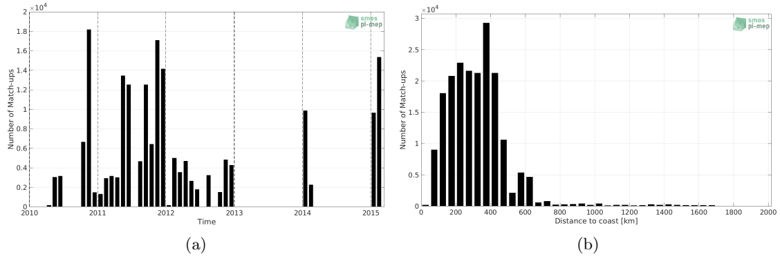
Figure 1: Number of match-ups between TSG (SAMOS) and SMOS L4 v2 Weekly (CATDS-CECOS-IFREMER) SSS as a function of time (a) and as function of the distance to coast (b) over the Roaring Forties and Furious Fifties Pi-MEP region and for the full satellite product period.
