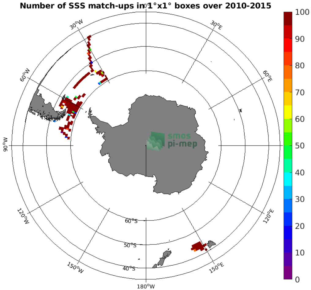
Figure 4: Number of SSS match-ups between TSG (SAMOS) SSS and the SMOS L4 v2 Weekly (CATDS-CECOS-IFREMER) SSS product for the Roaring Forties and Furious Fifties Pi-MEP region over 1^\circ \times 1^\circ boxes and for the full satellite product period.
