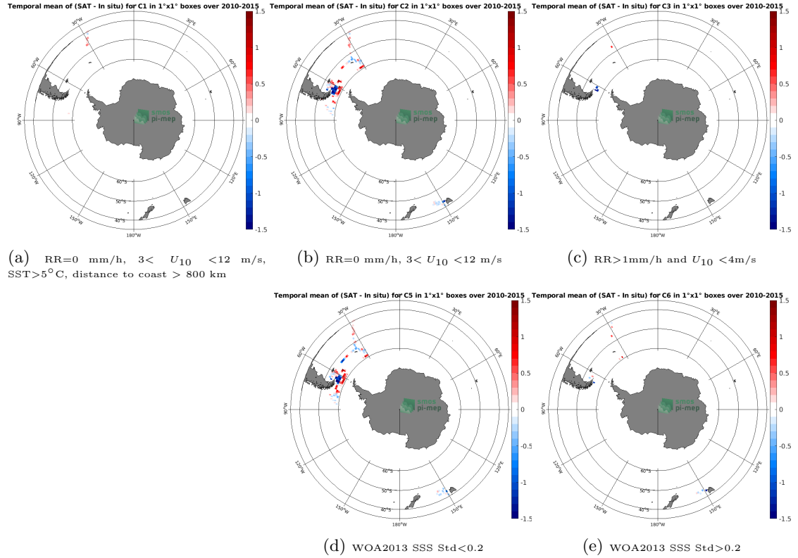
Figure 12: Temporal mean gridded over spatial boxes of size 1^{\circ}\times 1^{\circ} of \Delta\text{SSS} (SMOS L4 v2 Weekly (CATDS-CECOS-IFREMER) - TSG (SAMOS)) for 5 different subdatasets corresponding to: RR=0 mm/h, 3 < U_{10} < 12 m/s, SST > 5^{\circ}\text{C} , distance to coast > 800 km (a), RR=0 mm/h, 3 < U_{10} < 12 m/s (b), RR > 1 mm/h and U_{10} < 4 m/s (c), WOA2013 SSS Std < 0.2 (d), WOA2013 SSS Std > 0.2 (e).
