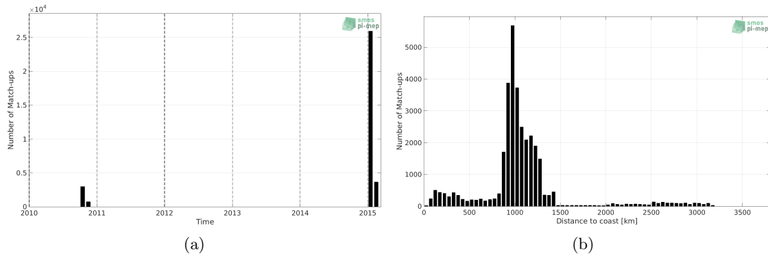
Figure 1: Number of match-ups between TSG (GOSUD-Research-vessel) and SMOS L4 v2 Weekly (CATDS-CECOS-IFREMER) SSS as a function of time (a) and as function of the distance to coast (b) over the Roaring Forties and Furious Fifties Pi-MEP region and for the full satellite product period.
