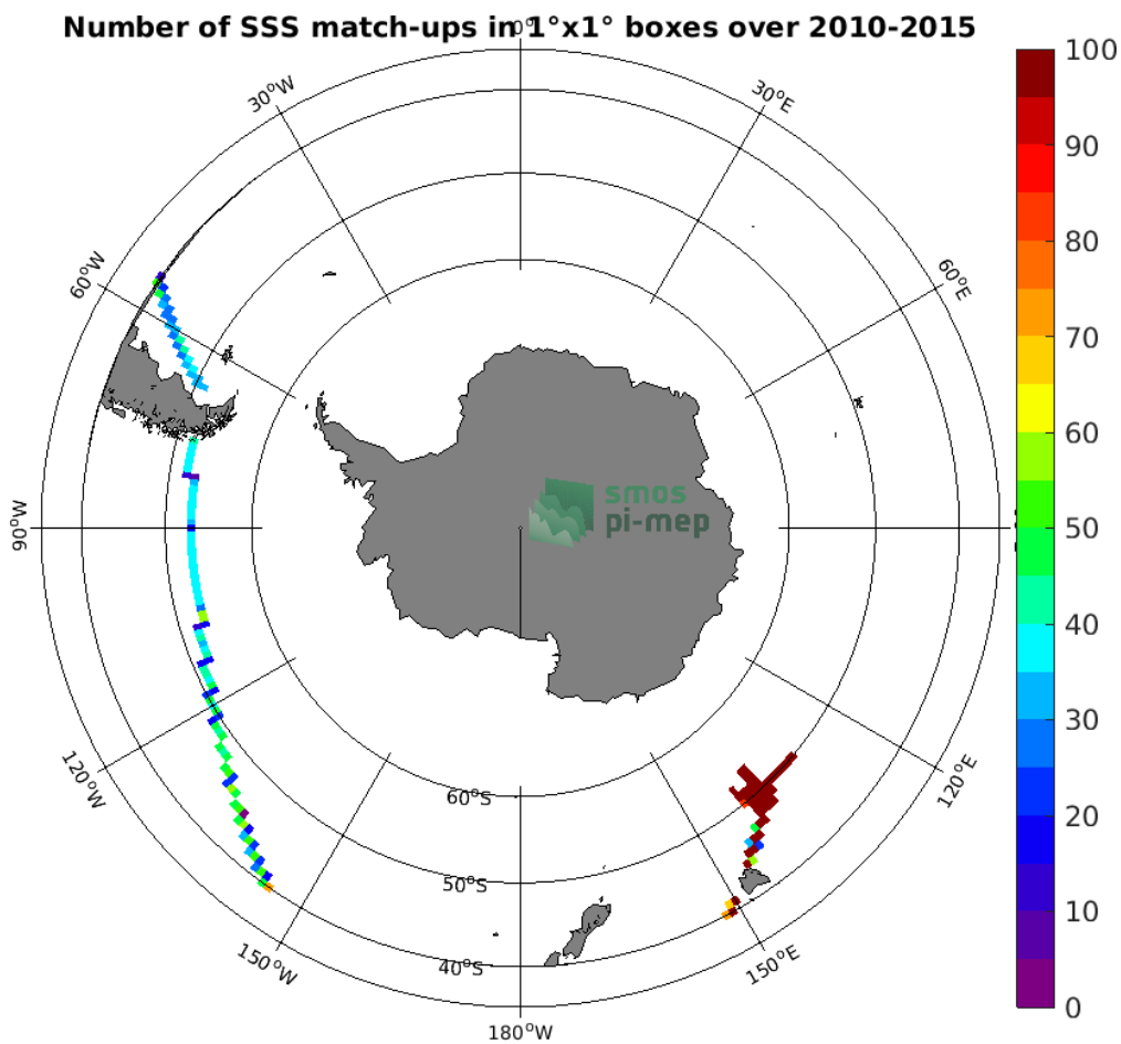
Figure 4: Number of SSS match-ups between TSG (GOSUD-Research-vessel) SSS and the SMOS L4 v2 Weekly (CATDS-CECOS-IFREMER) SSS product for the Roaring Forties and Furious Fifties Pi-MEP region over 1°x1° boxes and for the full satellite product period.
