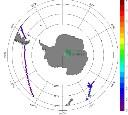
(f) Std( \Delta SSS) (Satellite - TSG (GOSUD-Research-vessel))
