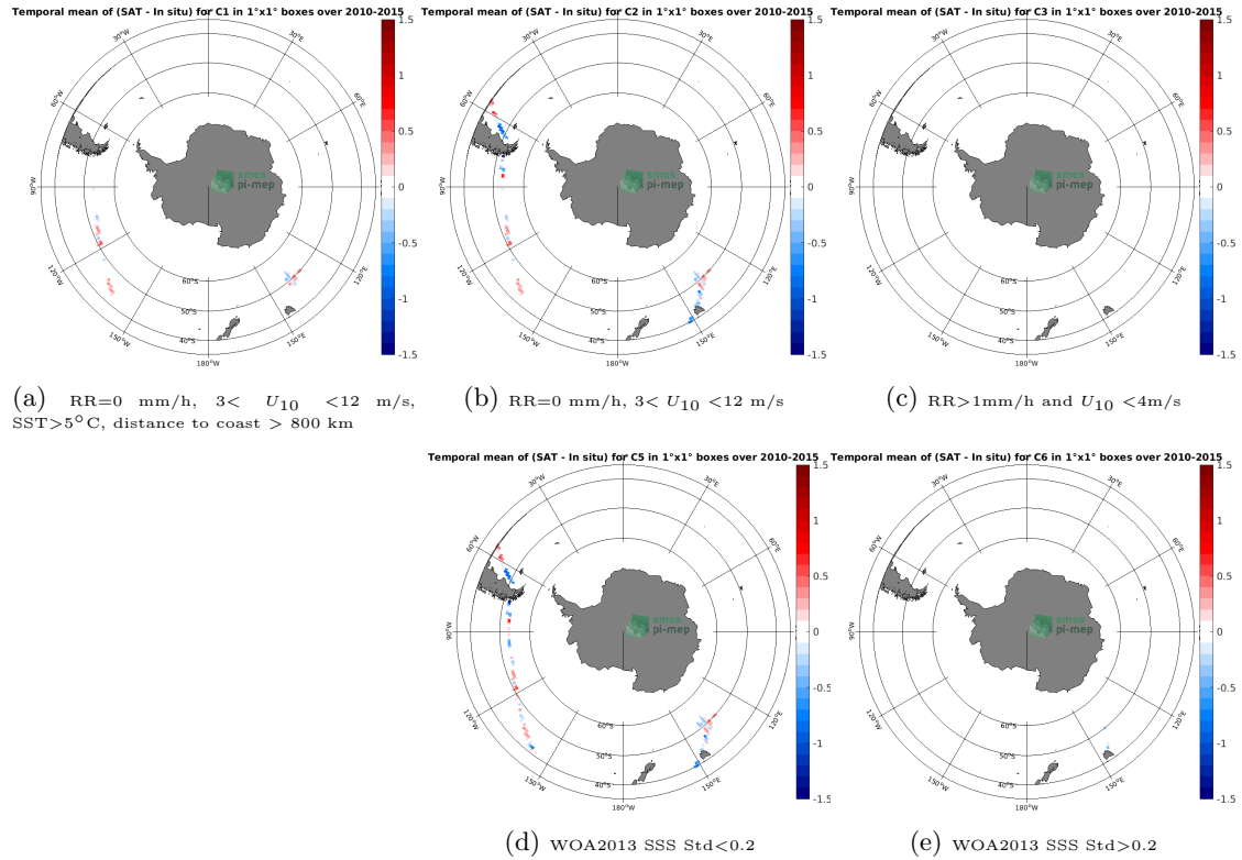
Figure 12: Temporal mean gridded over spatial boxes of size 1°x1° of \Delta SSS (SMOS L4 v2 Weekly (CATDS-CECOS-IFREMER) - TSG (GOSUD-Research-vessel)) for 5 different subdatasets corresponding to: RR=0 mm/h, 3 < U_{10} < 12 m/s, SST>5°C, distance to coast > 800 km (a), RR=0 mm/h, 3 < U_{10} < 12 m/s (b), RR>1mm/h and U_{10} < 4 m/s (c), WOA2013 SSS Std<0.2 (d), WOA2013 SSS Std>0.2 (e).
