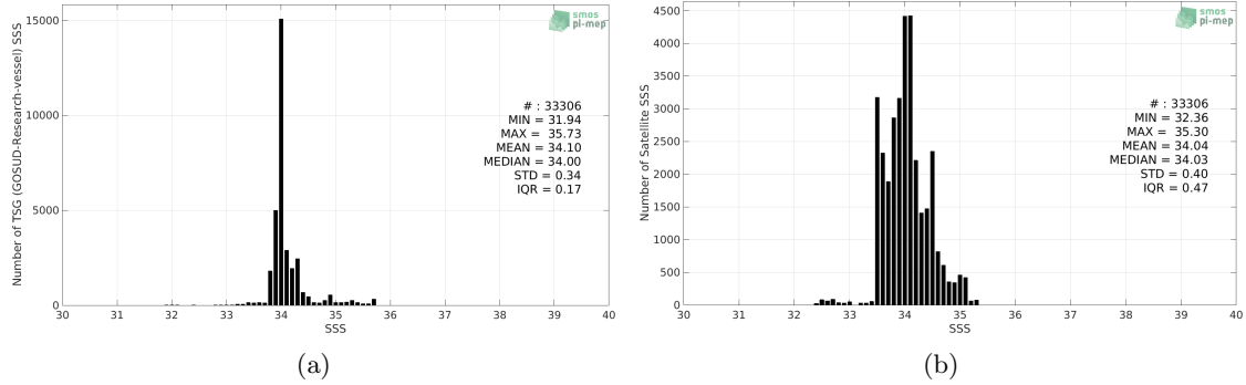
Figure 2: Histograms of SSS from TSG (GOSUD-Research-vessel) (a) and SMOS L4 v2 Weekly (CATDS-CECOS-IFREMER) (b) considering all match-up pairs per bins of 0.1 over the Roaring Forties and Furious Fifties Pi-MEP region and for the full satellite product period.
