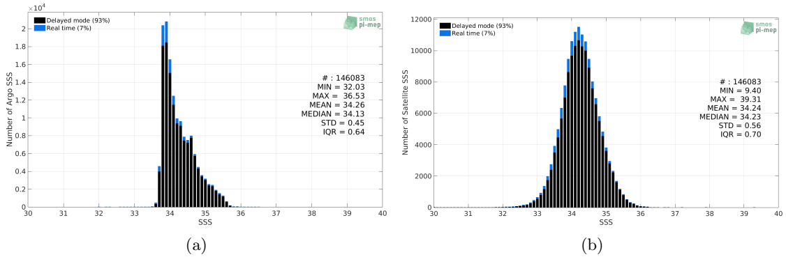
Figure 2: Histograms of SSS from Argo (a) and SMOS L4 v2 Weekly (CATDS-CECOS-IFREMER) (b) considering all match-up pairs per bins of 0.1 over the Roaring Forties and Furious Fifties Pi-MEP region and for the full satellite product period.
