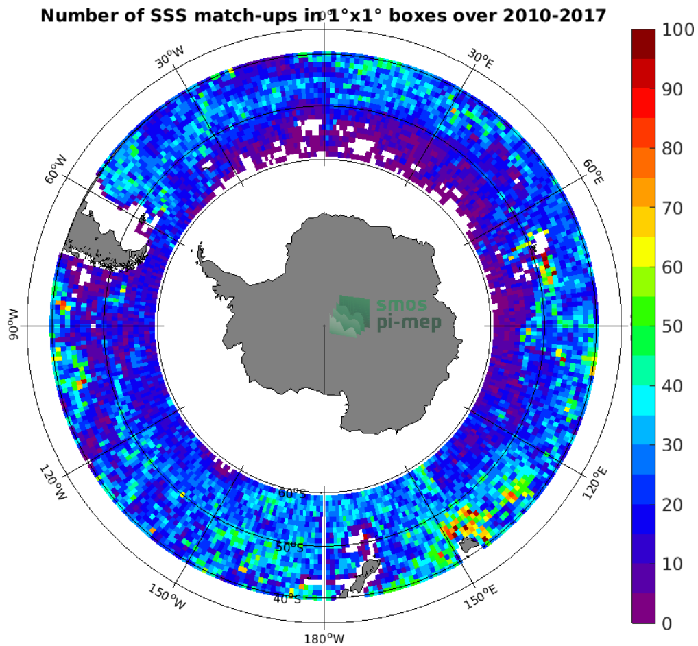
Figure 4: Number of SSS match-ups between Argo SSS and the SMOS L4 v2 Weekly (CATDS-CECOS-IFREMER) SSS product for the Roaring Forties and Furious Fifties Pi-MEP region over 1^\circ \times 1^\circ boxes and for the full satellite product period.
