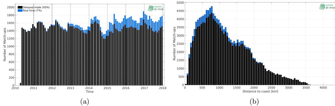
Figure 1: Number of match-ups between Argo and SMOS L4 v2 Weekly (CATDS-CECOS-IFREMER) SSS as a function of time (a) and as function of the distance to coast (b) over the Roaring Forties and Furious Fifties Pi-MEP region and for the full satellite product period.
