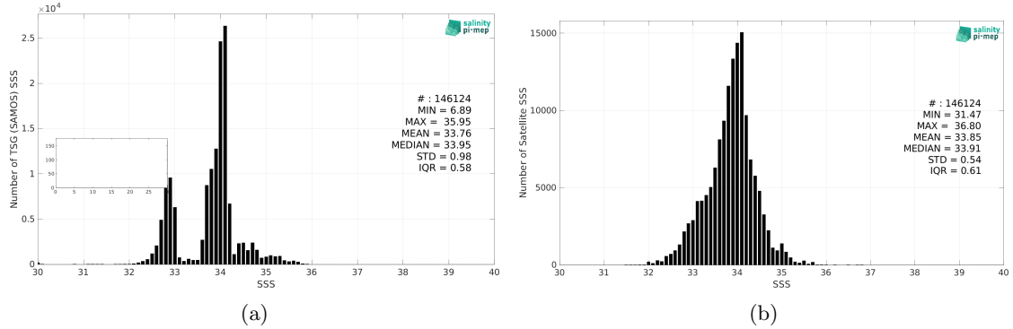
Figure 2: Histograms of SSS from TSG (SAMOS) (a) and SMOS SSS L4 v2 - Daily (BEC) (b) considering all match-up pairs per bins of 0.1 over the Roaring Forties and Furious Fifties Pi-MEP region and for the full satellite product period.
