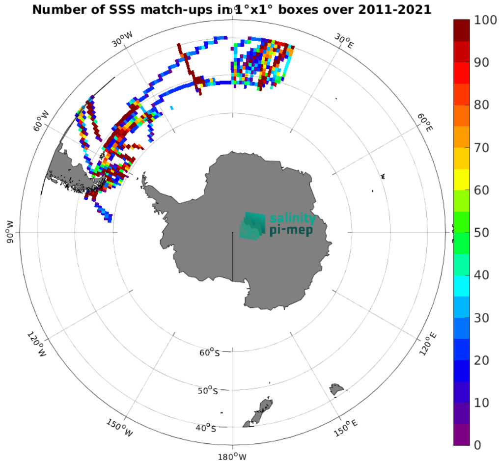
Figure 4: Number of SSS match-ups between TSG (Polarstern) SSS and the SMOS SSS L4 v2 - Daily (BEC) SSS product for the Roaring Forties and Furious Fifties Pi-MEP region over 1^\circ \times 1^\circ boxes and for the full satellite product period.
