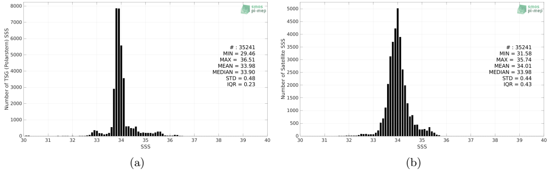
Figure 2: Histograms of SSS from TSG (Polarstern) (a) and SMOS SSS L4 v2 - Daily (BEC) (b) considering all match-up pairs per bins of 0.1 over the Roaring Forties and Furious Fifties Pi-MEP region and for the full satellite product period.
