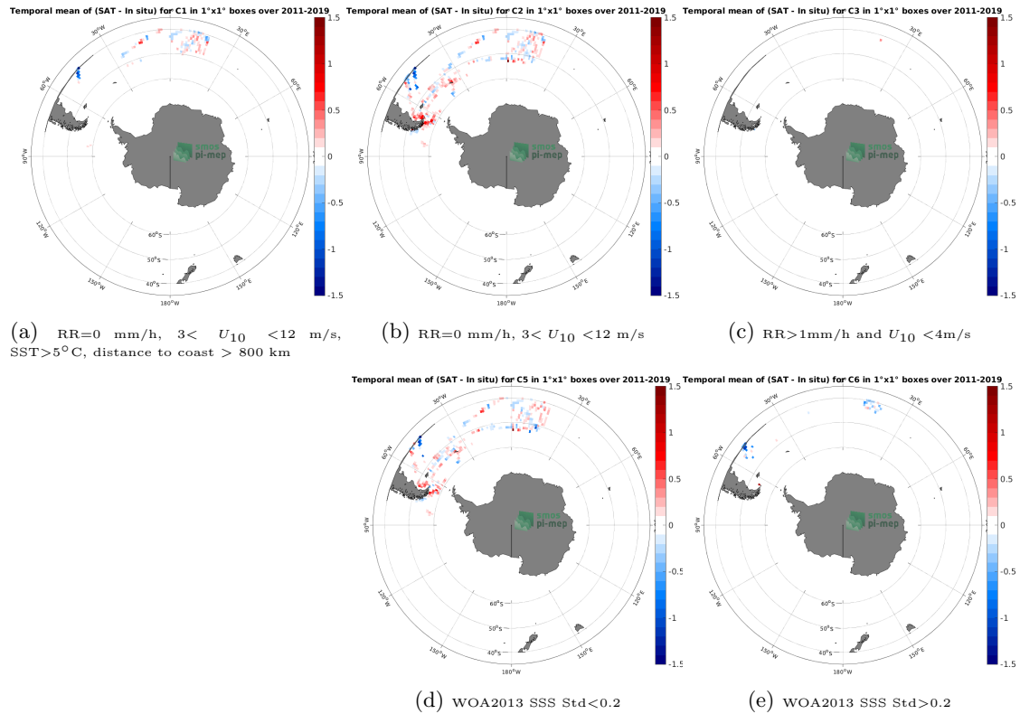
Figure 12: Temporal mean gridded over spatial boxes of size 1^{\circ}\times 1^{\circ} of \Delta\text{SSS} (SMOS SSS L4 v2 - Daily (BEC) - TSG (Polarstern)) for 5 different subdatasets corresponding to:RR=0 mm/h, 3 < U_{10} < 12 m/s, SST >5^{\circ}\text{C} , distance to coast > 800 km (a), RR=0 mm/h, 3 < U_{10} < 12 m/s (b), RR >1 mm/h and U_{10} < 4 m/s (c), WOA2013 SSS Std <0.2 (d), WOA2013 SSS Std >0.2 (e).
