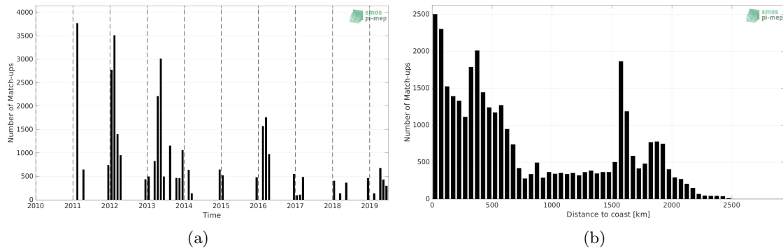
Figure 1: Number of match-ups between TSG (Polarstern) and SMOS SSS L4 v2 - Daily (BEC) SSS as a function of time (a) and as function of the distance to coast (b) over the Roaring Forties and Furious Fifties Pi-MEP region and for the full satellite product period.
