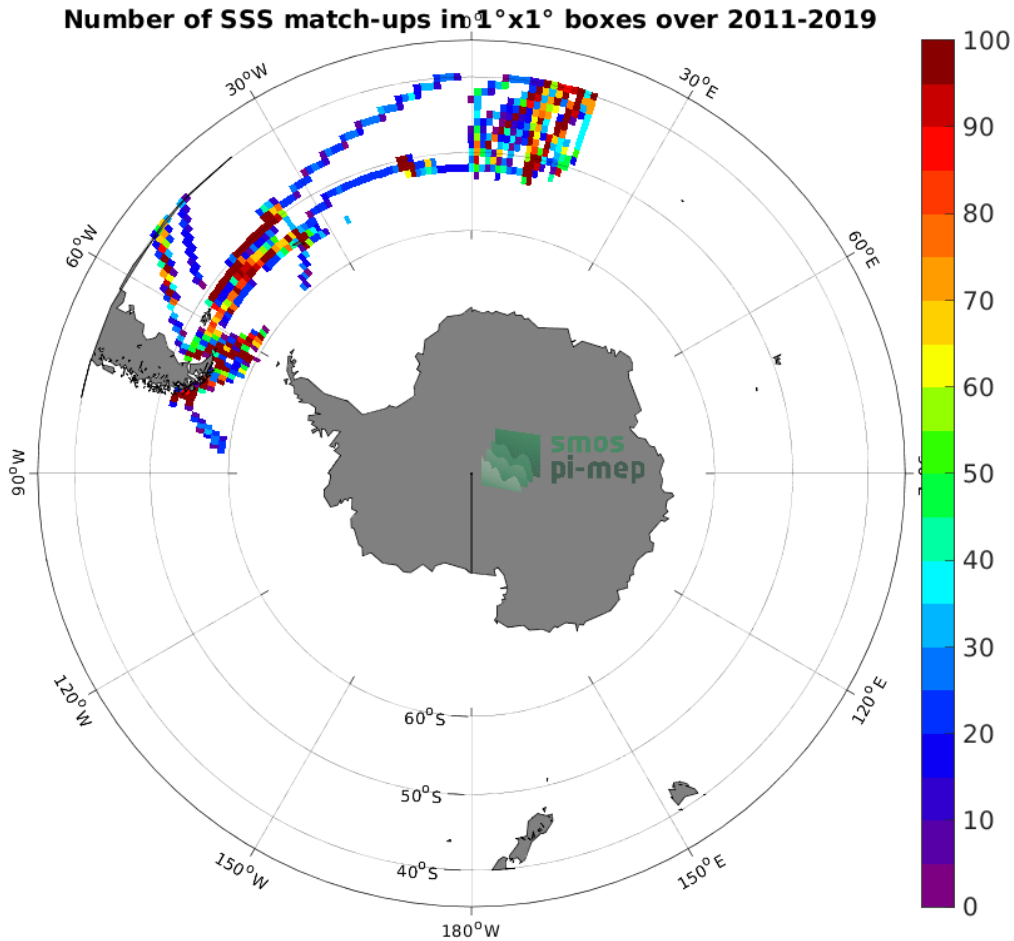
Figure 4: Number of SSS match-ups between TSG (Polarstern) SSS and the SMOS SSS L4 v2 - Daily (BEC) SSS product for the Roaring Forties and Furious Fifties Pi-MEP region over 1^\circ \times 1^\circ boxes and for the full satellite product period.
