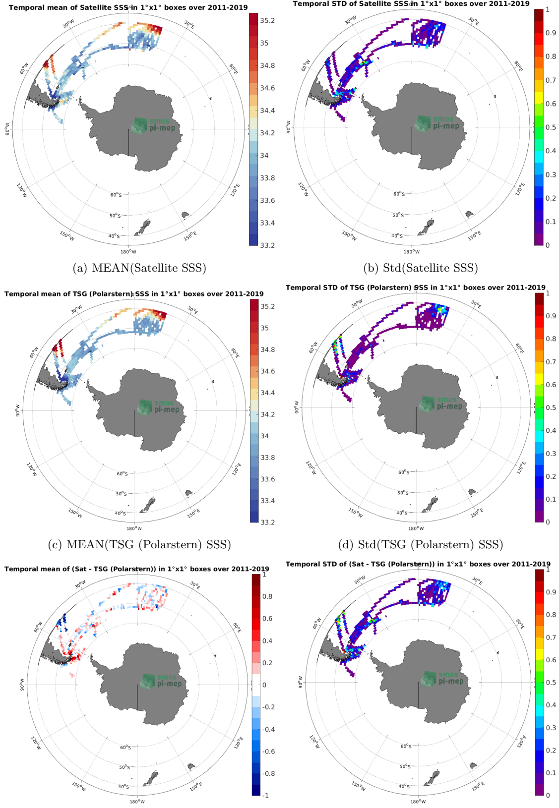
Figure 6: Temporal mean (left) and Std (right) of SSS from SMOS SSS L4 v2 - Daily (BEC) (top), TSG (Polarstern) (middle), and of \Delta SSS (Satellite - TSG (Polarstern)). Only match-up pairs are used to generate these maps.
