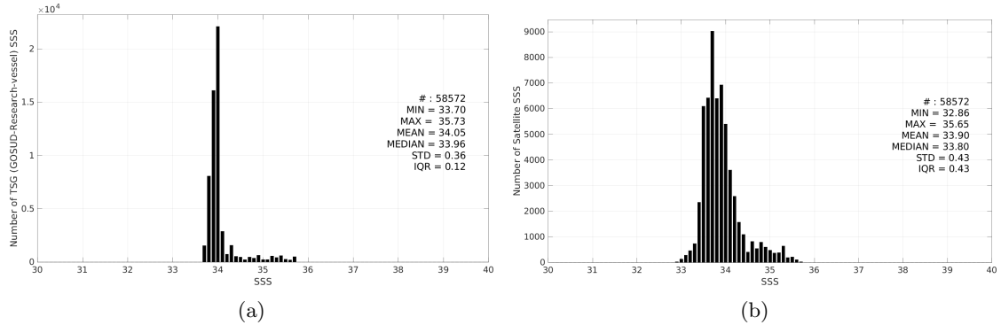
Figure 3: Histograms of SSS from TSG (GOSUD-Research-vessel) (a) and SMOS SSS L4 v2 - Daily (BEC) (b) considering all match-up pairs per bins of 0.1 over the Roaring Forties and Furious Fifties Pi-MEP region and for the full satellite product period.
