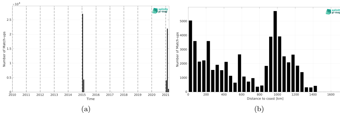
Figure 2: Number of match-ups between TSG (GOSUD-Research-vessel) and SMOS SSS L4 v2 - Daily (BEC) SSS as a function of time (a) and as function of the distance to coast (b) over the Roaring Forties and Furious Fifties Pi-MEP region and for the full satellite product period.
