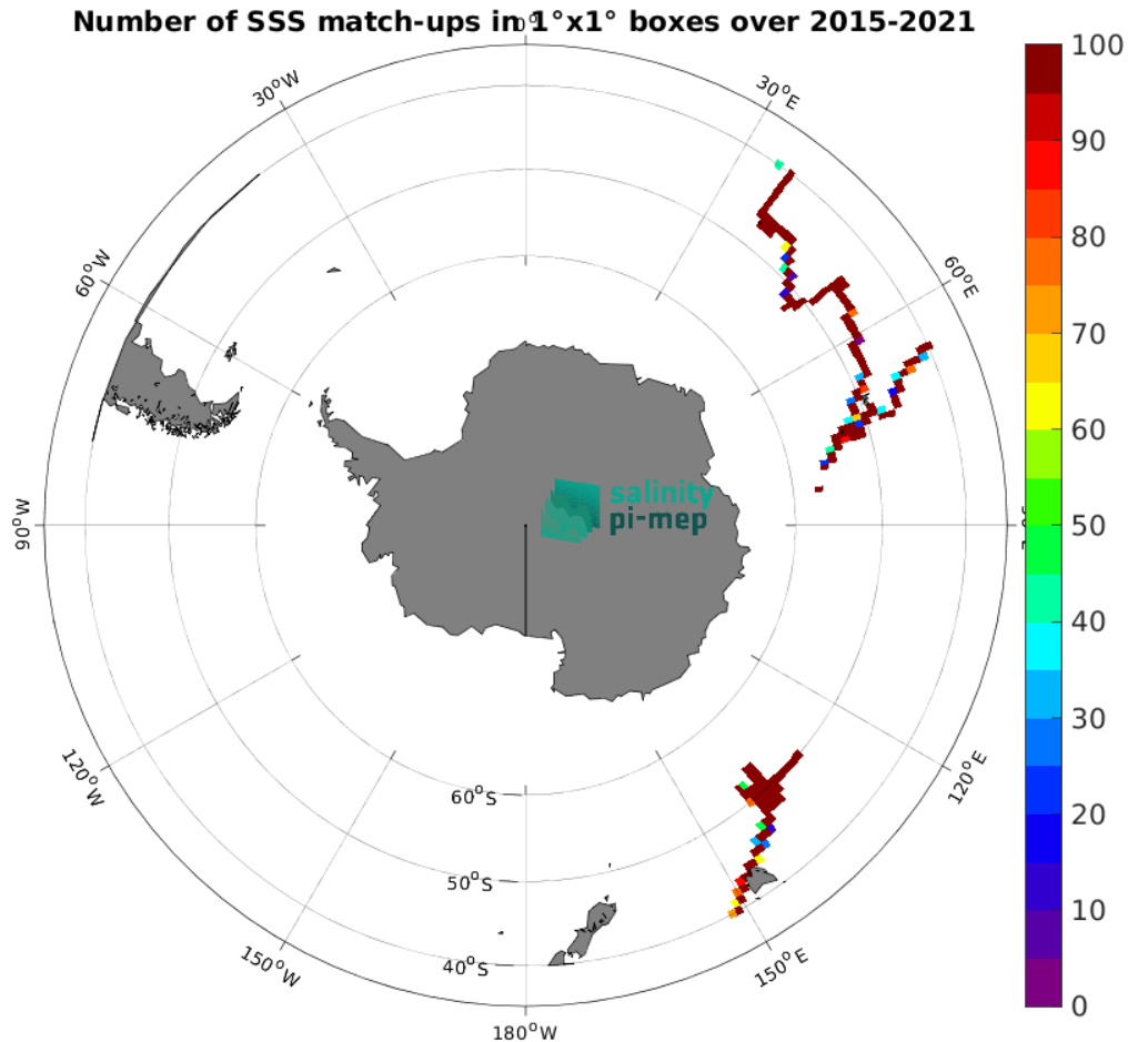
Figure 5: Number of SSS match-ups between TSG (GOSUD-Research-vessel) SSS and the SMOS SSS L4 v2 - Daily (BEC) SSS product for the Roaring Forties and Furious Fifties Pi-MEP region over 1^\circ \times 1^\circ boxes and for the full satellite product period.
