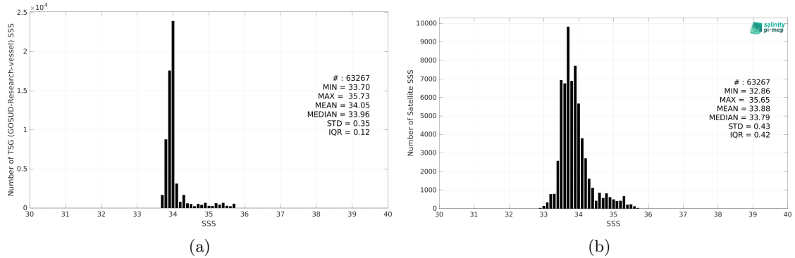
Figure 2: Histograms of SSS from TSG (GOSUD-Research-vessel) (a) and SMOS SSS L4 v2 - Daily (BEC) (b) considering all match-up pairs per bins of 0.1 over the Roaring Forties and Furious Fifties Pi-MEP region and for the full satellite product period.
