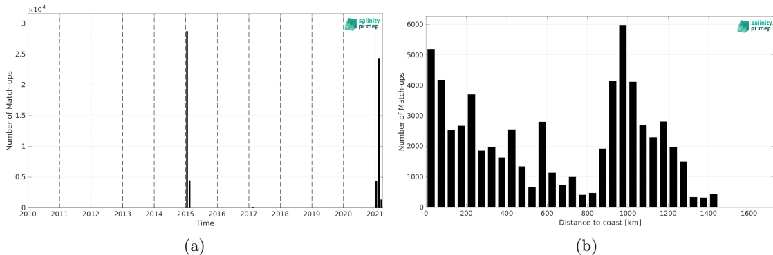
Figure 1: Number of match-ups between TSG (GOSUD-Research-vessel) and SMOS SSS L4 v2 - Daily (BEC) SSS as a function of time (a) and as function of the distance to coast (b) over the Roaring Forties and Furious Fifties Pi-MEP region and for the full satellite product period.
