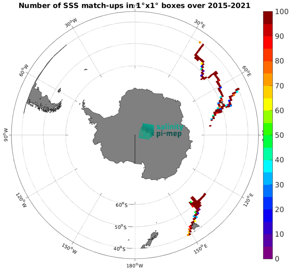
Figure 4: Number of SSS match-ups between TSG (GOSUD-Research-vessel) SSS and the SMOS SSS L4 v2 - Daily (BEC) SSS product for the Roaring Forties and Furious Fifties Pi-MEP region over 1^\circ \times 1^\circ boxes and for the full satellite product period.
