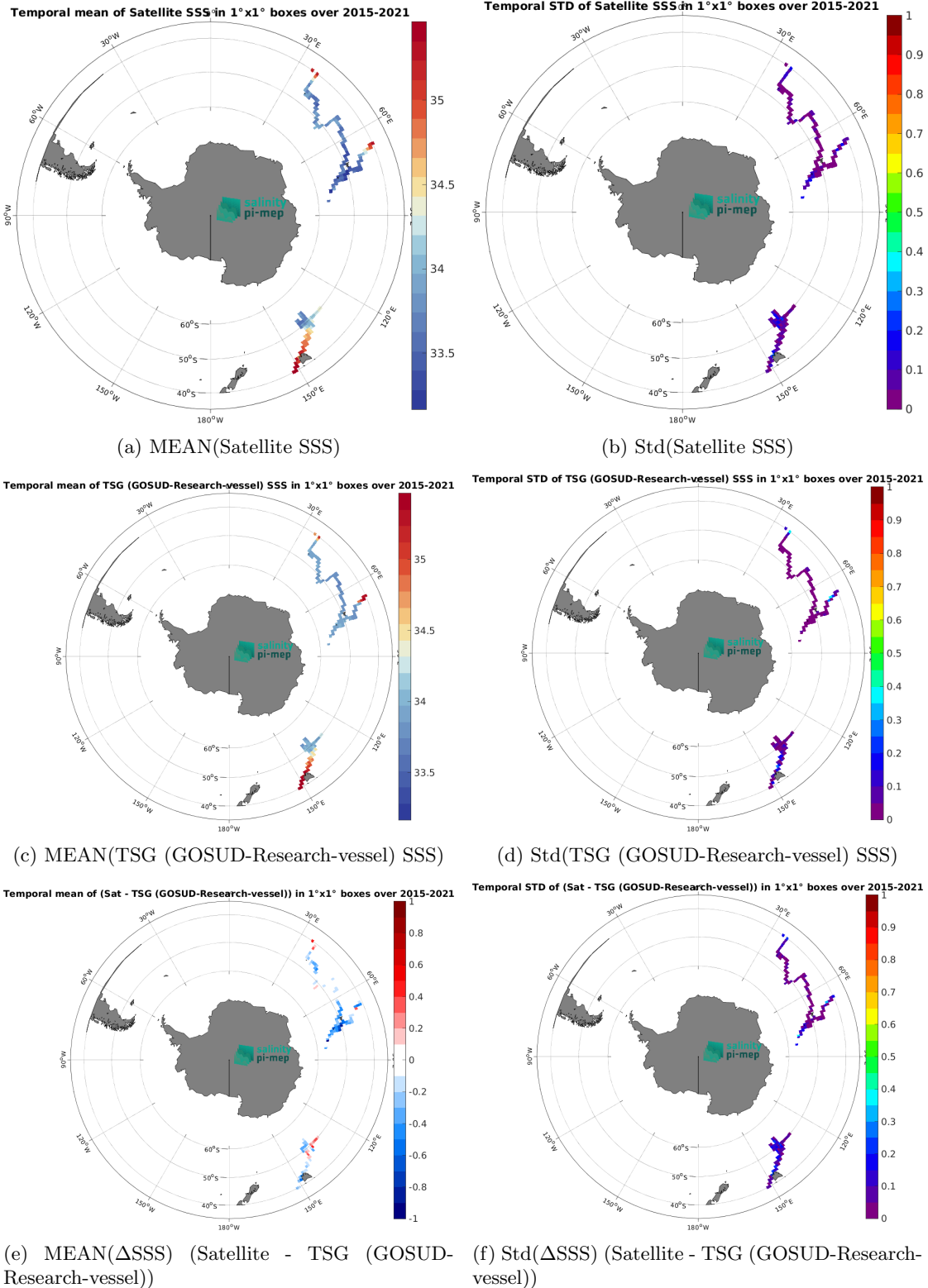
Figure 6: Temporal mean (left) and Std (right) of SSS from SMOS SSS L4 v2 - Daily (BEC) (top), TSG (GOSUD-Research-vessel) (middle), and of \Delta SSS (Satellite - TSG (GOSUD-Research-vessel)). Only match-up pairs are used to generate these maps.
