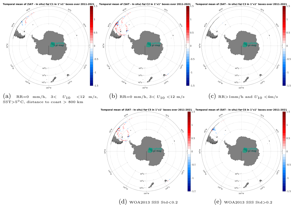
Figure 14: Temporal mean gridded over spatial boxes of size 1^\circ \times 1^\circ of \Delta SSS (SMOS SSS L4 v2 - Daily (BEC) - TSG (CSIC-UTM)) for 5 different subdatasets corresponding to:RR=0 mm/h, 3 < U_{10} < 12 m/s, SST >5^\circ C, distance to coast > 800 km (a), RR=0 mm/h, 3 < U_{10} < 12 m/s (b), RR >1 mm/h and U_{10} < 4 m/s (c), WOA2013 SSS Std <0.2 (d), WOA2013 SSS Std >0.2 (e).
