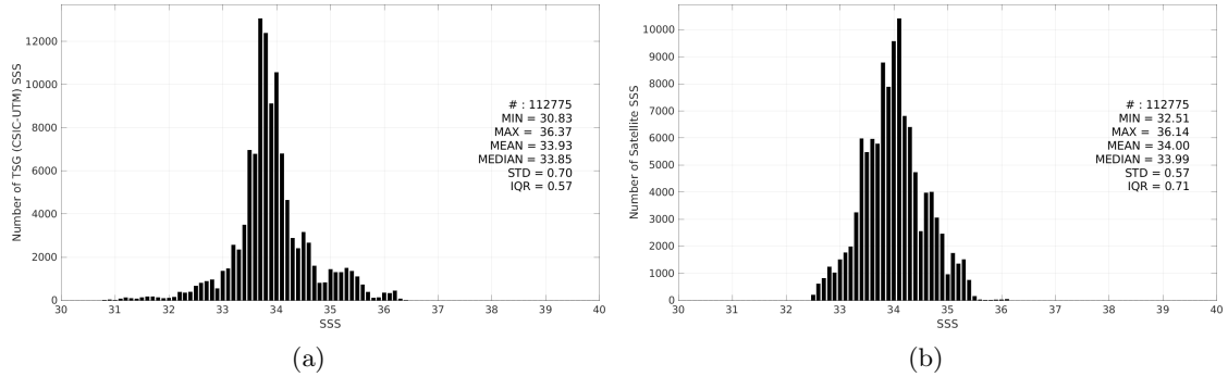
Figure 3: Histograms of SSS from TSG (CSIC-UTM) (a) and SMOS SSS L4 v2 - Daily (BEC) (b) considering all match-up pairs per bins of 0.1 over the Roaring Forties and Furious Fifties Pi-MEP region and for the full satellite product period.
