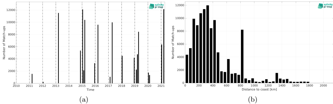
Figure 2: Number of match-ups between TSG (CSIC-UTM) and SMOS SSS L4 v2 - Daily (BEC) SSS as a function of time (a) and as function of the distance to coast (b) over the Roaring Forties and Furious Fifties Pi-MEP region and for the full satellite product period.
