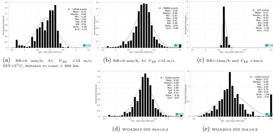
Figure 15: Normalized histogram of \Delta\text{SSS} (SMOS SSS L4 v2 - Daily (BEC) - TSG (CSIC-UTM)) for 5 different subdatasets corresponding to: RR=0 mm/h, 3 < U_{10} < 12 m/s, SST>5°C, distance to coast > 800 km (a), RR=0 mm/h, 3 < U_{10} < 12 m/s (b), RR>1mm/h and U_{10} < 4 m/s (c), WOA2013 SSS Std<0.2 (d), WOA2013 SSS Std>0.2 (e).
