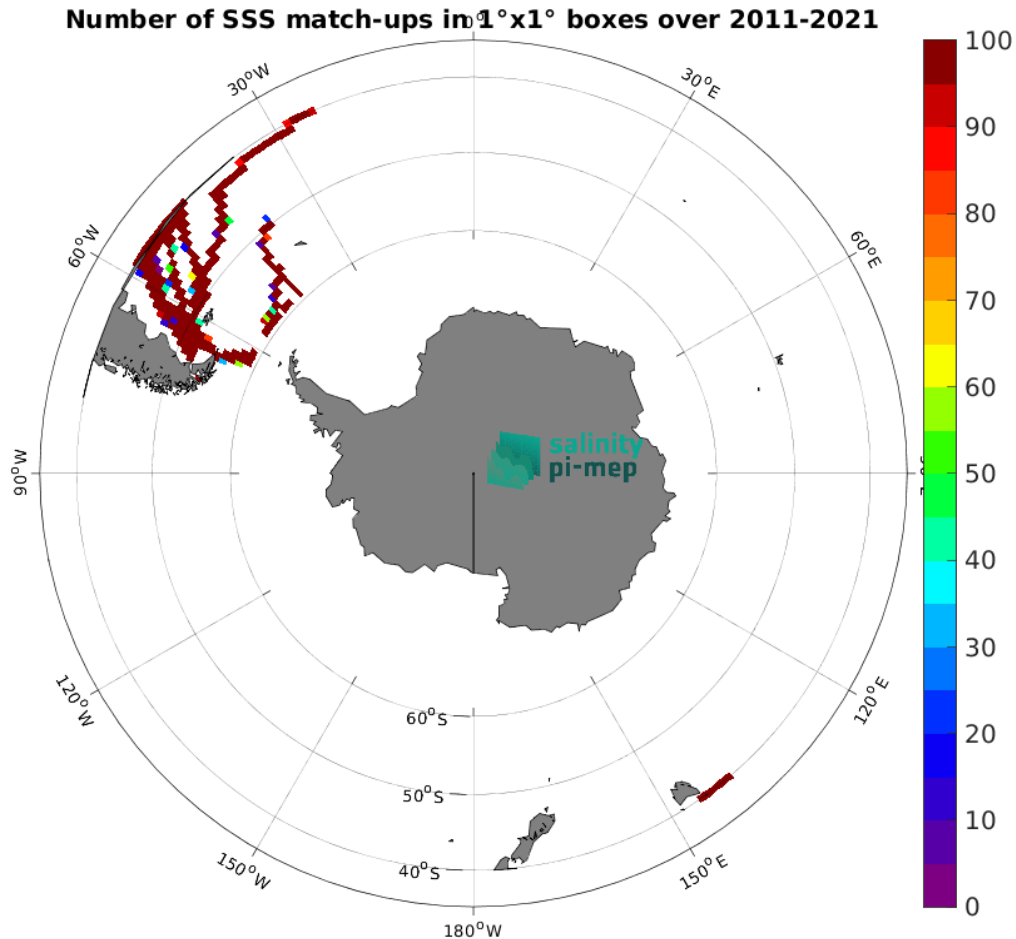
Figure 5: Number of SSS match-ups between TSG (CSIC-UTM) SSS and the SMOS SSS L4 v2 - Daily (BEC) SSS product for the Roaring Forties and Furious Fifties Pi-MEP region over 1^\circ \times 1^\circ boxes and for the full satellite product period.
