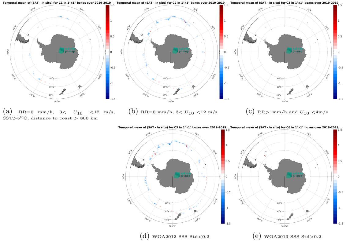
Figure 12: Temporal mean gridded over spatial boxes of size 1^{\circ}\times 1^{\circ} of \Delta\text{SSS} (SMOS SSS L4 v2 - Daily (BEC) - Sairdrone) for 5 different subdatasets corresponding to: \text{RR}=0 mm/h, 3 < U_{10} < 12 m/s, \text{SST}>5^{\circ}\text{C} , distance to coast > 800 km (a), \text{RR}=0 mm/h, 3 < U_{10} < 12 m/s (b), \text{RR}>1\text{mm/h} and U_{10} < 4\text{m/s} (c), WOA2013 SSS Std <0.2 (d), WOA2013 SSS Std >0.2 (e).
