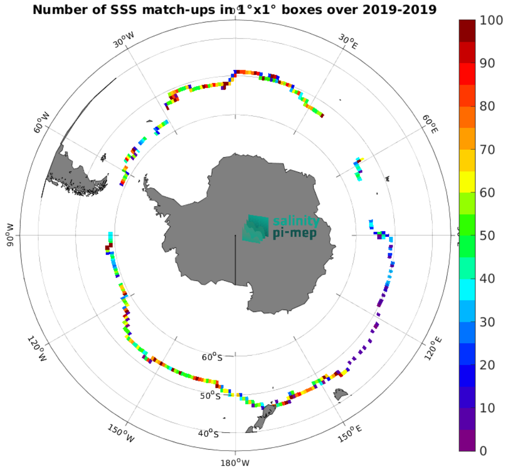
Figure 4: Number of SSS match-ups between Saildrone SSS and the SMOS SSS L4 v2 - Daily (BEC) SSS product for the Roaring Forties and Furious Fifties Pi-MEP region over 1^\circ \times 1^\circ boxes and for the full satellite product period.
