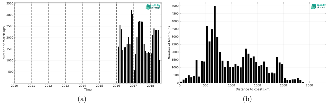
Figure 2: Number of match-ups between Surface drifters and SMOS SSS L4 v2 - Daily (BEC) SSS as a function of time (a) and as function of the distance to coast (b) over the Roaring Forties and Furious Fifties Pi-MEP region and for the full satellite product period.
