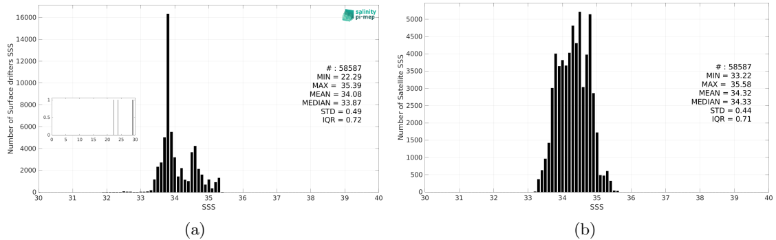
Figure 3: Histograms of SSS from Surface drifters (a) and SMOS SSS L4 v2 - Daily (BEC) (b) considering all match-up pairs per bins of 0.1 over the Roaring Forties and Furious Fifties Pi-MEP region and for the full satellite product period.
