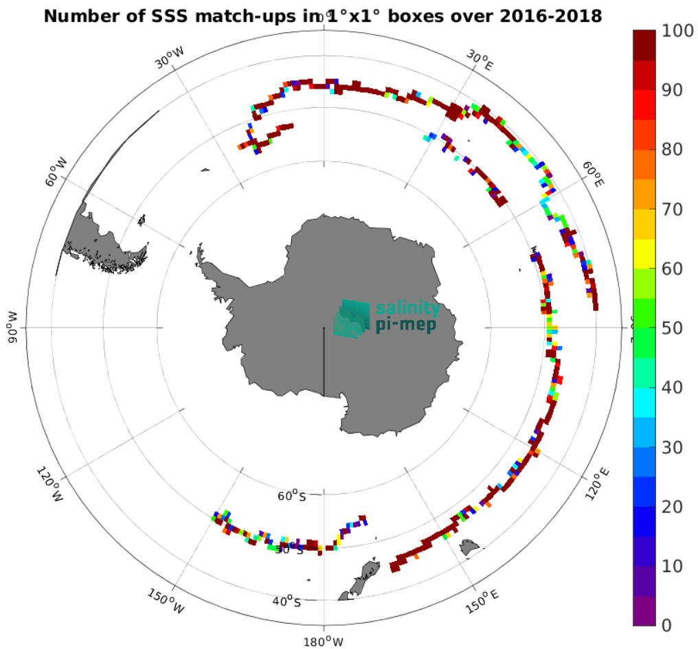
Figure 4: Number of SSS match-ups between Surface drifters SSS and the SMOS SSS L4 v2 - Daily (BEC) SSS product for the Roaring Forties and Furious Fifties Pi-MEP region over 1^\circ \times 1^\circ boxes and for the full satellite product period.
