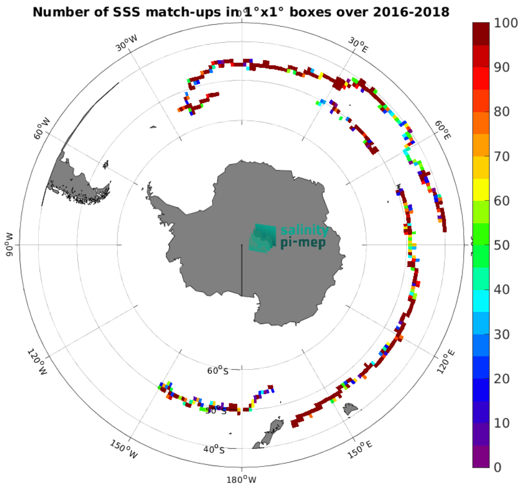
Figure 3: Number of SSS match-ups between Surface drifters SSS and the SMOS SSS L4 v2 - Daily (BEC) SSS product for the Roaring Forties and Furious Fifties Pi-MEP region over 1^\circ \times 1^\circ boxes and for the full satellite product period.
