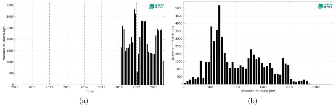
Figure 1: Number of match-ups between Surface drifters and SMOS SSS L4 v2 - Daily (BEC) SSS as a function of time (a) and as function of the distance to coast (b) over the Roaring Forties and Furious Fifties Pi-MEP region and for the full satellite product period.
