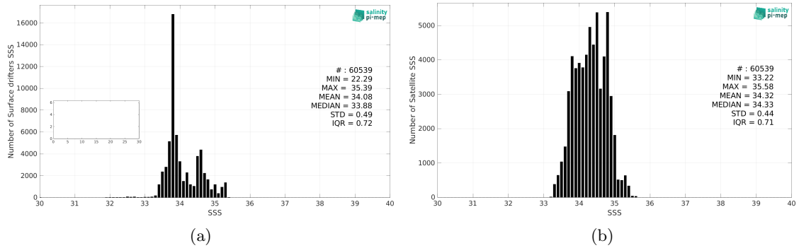
Figure 2: Histograms of SSS from Surface drifters (a) and SMOS SSS L4 v2 - Daily (BEC) (b) considering all match-up pairs per bins of 0.1 over the Roaring Forties and Furious Fifties Pi-MEP region and for the full satellite product period.
