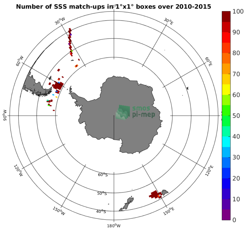
Figure 4: Number of SSS match-ups between TSG-SAMOS SSS and the SMOS-L3-ICDC-V3-MONTHLY-0.5DEG SSS product for the Roaring Forties and Furious Fifties Pi-MEP region over 1^\circ \times 1^\circ boxes and for the full satellite product period.
