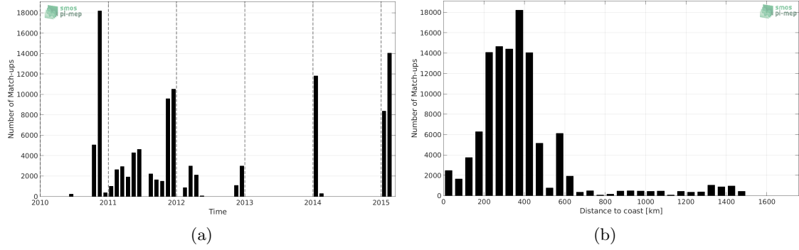
Figure 1: Number of match-ups between TSG-SAMOS and SMOS-L3-ICDC-V3-MONTHLY-0.5DEG SSS as a function of time (a) and as function of the distance to coast (b) over the Roaring Forties and Furious Fifties Pi-MEP region and for the full satellite product period.
