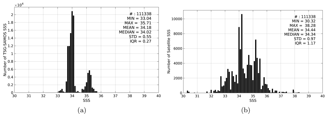
Figure 2: Histograms of SSS from TSG-SAMOS (a) and SMOS-L3-ICDC-V3-MONTHLY-0.5DEG (b) considering all match-up pairs per bins of 0.1 over the Roaring Forties and Furious Fifties Pi-MEP region and for the full satellite product period.
