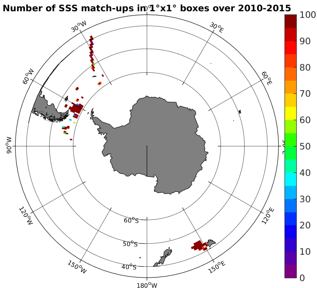
Figure 4: Number of SSS match-ups between TSG-SAMOS SSS and the SMOS-L3-ICDC-V3-MONTHLY-0.5DEG SSS product for the Roaring Forties and Furious Fifties Pi-MEP region over 1^\circ \times 1^\circ boxes and for the full satellite product period.
