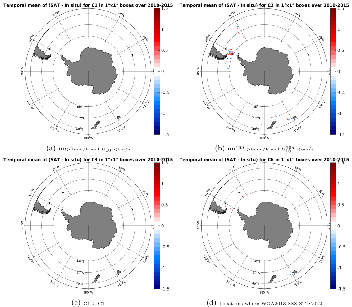
Figure 12: Temporal mean gridded over spatial boxes of size 1^\circ \times 1^\circ of \Delta SSS (SMOS-L3-ICDC-V3-MONTHLY-0.5DEG - TSG-SAMOS) for 4 different subdatasets corresponding to: RR > 1\text{mm/h} and U_{10} < 5\text{m/s} (a), RR^{10d} > 5\text{mm/h} and U_{10}^{10d} < 5\text{m/s} (b), C1 U C2 (c), Locations where WOA2013 SSS STD > 0.2 (d).
