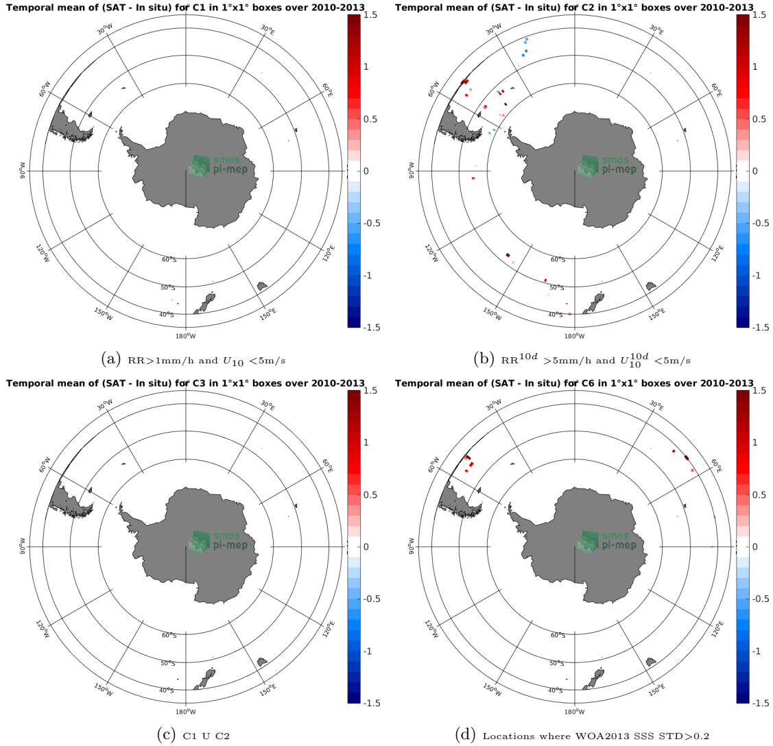
Figure 12: Temporal mean gridded over spatial boxes of size 1^\circ \times 1^\circ of \Delta SSS (SMOS-L3-ICDC-V3-MONTHLY-0.5DEG - TSG-GOSUD-Sailing-ship) for 4 different subdatasets corresponding to: RR > 1\text{mm/h} and U_{10} < 5\text{m/s} (a), RR^{10d} > 5\text{mm/h} and U_{10}^{10d} < 5\text{m/s} (b), C1 U C2 (c), Locations where WOA2013 SSS STD > 0.2 (d).
