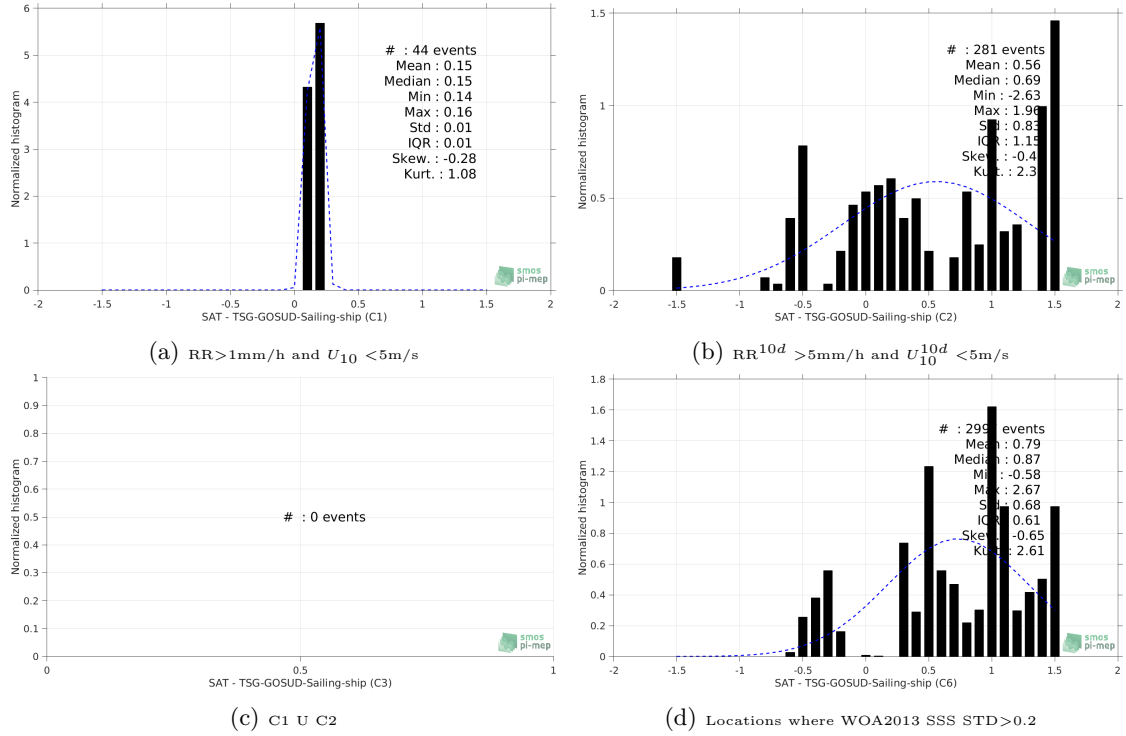
Figure 13: Normalized histogram of \Delta\text{SSS} (SMOS-L3-ICDC-V3-MONTHLY-0.5DEG - TSG-GOSUD-Sailing-ship) for 6 different subdatasets corresponding to: RR > 1mm/h and U_{10} < 5\text{m/s} (a), RR^{10d} > 5\text{mm/h} and U_{10}^{10d} < 5\text{m/s} (b), C1 U C2 (c), Locations where WOA2013 SSS STD > 0.2 (d).
