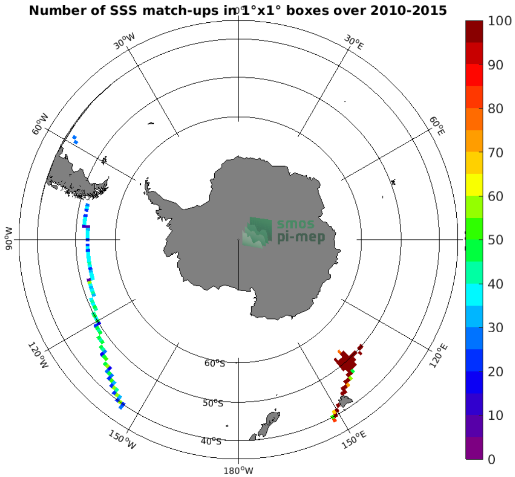
Figure 4: Number of SSS match-ups between TSG (GOSUD-Research-vessel) SSS and the SMOS SSS L3 v3 Monthly (ICDC) SSS product for the Roaring Forties and Furious Fifties Pi-MEP region over 1°x1° boxes and for the full satellite product period.
