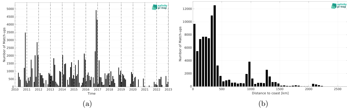
Figure 2: Number of match-ups between TSG (SAMOS) and SMOS SSS L2Q v331 - With FLAG (CMEMS-CATDS-CPDC) SSS as a function of time (a) and as function of the distance to coast (b) over the Roaring Forties and Furious Fifties Pi-MEP region and for the full satellite product period.
