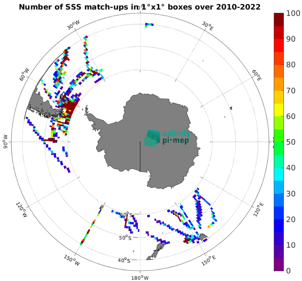
Figure 5: Number of SSS match-ups between TSG (SAMOS) SSS and the SMOS SSS L2Q v331 - With FLAG (CMEMS-CATDS-CPDC) SSS product for the Roaring Forties and Furious Fifties Pi-MEP region over 1^\circ \times 1^\circ boxes and for the full satellite product period.
