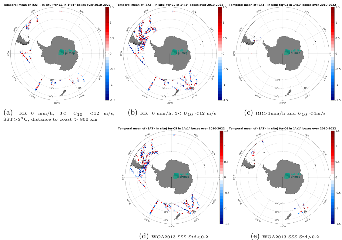
Figure 14: Temporal mean gridded over spatial boxes of size 1^\circ \times 1^\circ of \Delta SSS (SMOS SSS L2Q v331 - With FLAG (CMEMS-CATDS-CPDC) - TSG (SAMOS)) for 5 different subdatasets corresponding to: RR=0 mm/h, 3 < U_{10} < 12 m/s, SST > 5°C, distance to coast > 800 km (a), RR=0 mm/h, 3 < U_{10} < 12 m/s (b), RR > 1mm/h and U_{10} < 4 m/s (c), WOA2013 SSS Std < 0.2 (d), WOA2013 SSS Std > 0.2 (e).
