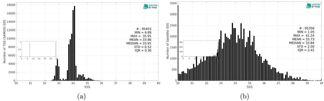
Figure 3: Histograms of SSS from TSG (SAMOS) (a) and SMOS SSS L2Q v331 - With FLAG (CMEMS-CATDS-CPDC) (b) considering all match-up pairs per bins of 0.1 over the Roaring Forties and Furious Fifties Pi-MEP region and for the full satellite product period.
