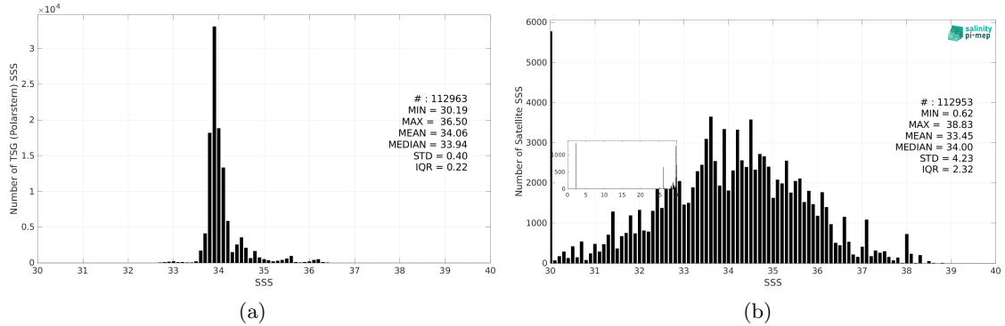
Figure 3: Histograms of SSS from TSG (Polarstern) (a) and SMOS SSS L2Q v331 - With FLAG (CMEMS-CATDS-CPDC) (b) considering all match-up pairs per bins of 0.1 over the Roaring Forties and Furious Fifties Pi-MEP region and for the full satellite product period.
