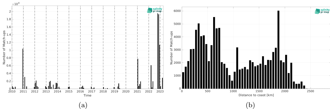
Figure 2: Number of match-ups between TSG (Polarstern) and SMOS SSS L2Q v331 - With FLAG (CMEMS-CATDS-CPDC) SSS as a function of time (a) and as function of the distance to coast (b) over the Roaring Forties and Furious Fifties Pi-MEP region and for the full satellite product period.
