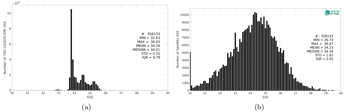
Figure 2: Histograms of SSS from TSG (LEGOS-DM) (a) and SMOS SSS L2Q v331 - With FLAG (CMEMS-CATDS-CPDC) (b) considering all match-up pairs per bins of 0.1 over the Roaring Forties and Furious Fifties Pi-MEP region and for the full satellite product period.
