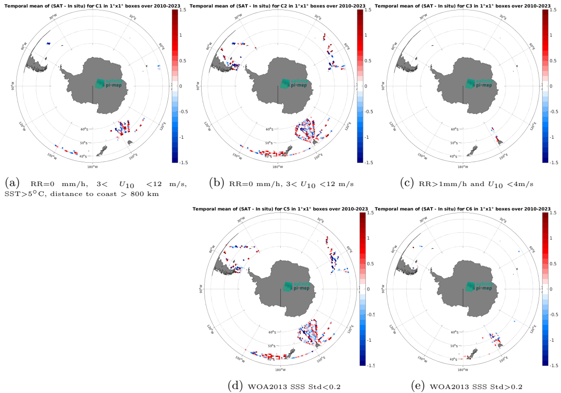
Figure 12: Temporal mean gridded over spatial boxes of size 1^{\circ}\times 1^{\circ} of \Delta\text{SSS} (SMOS SSS L2Q v331 - With FLAG (CMEMS-CATDS-CPDC) - TSG (LEGOS-DM)) for 5 different subdatasets corresponding to:RR=0 mm/h, 3 < U_{10} < 12 m/s, SST > 5^{\circ}\text{C} , distance to coast > 800 km (a), RR=0 mm/h, 3 < U_{10} < 12 m/s (b), RR > 1 mm/h and U_{10} < 4 m/s (c), WOA2013 SSS Std < 0.2 (d), WOA2013 SSS Std > 0.2 (e).
