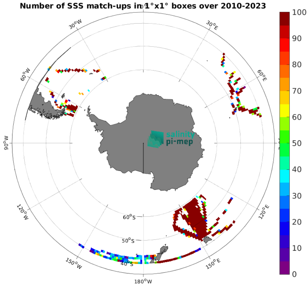
Figure 4: Number of SSS match-ups between TSG (LEGOS-DM) SSS and the SMOS SSS L2Q v331 - With FLAG (CMEMS-CATDS-CPDC) SSS product for the Roaring Forties and Furious Fifties Pi-MEP region over 1^\circ \times 1^\circ boxes and for the full satellite product period.
