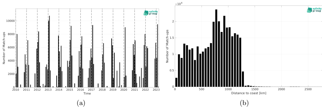
Figure 1: Number of match-ups between TSG (LEGOS-DM) and SMOS SSS L2Q v331 - With FLAG (CMEMS-CATDS-CPDC) SSS as a function of time (a) and as function of the distance to coast (b) over the Roaring Forties and Furious Fifties Pi-MEP region and for the full satellite product period.
