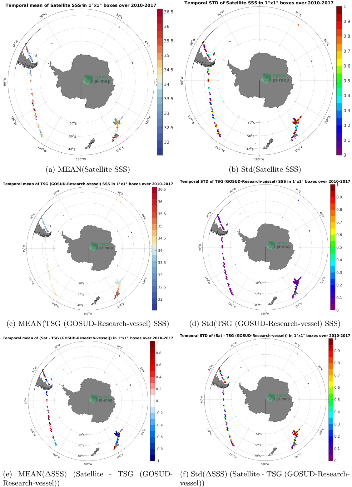
Figure 6: Temporal mean (left) and Std (right) of SSS from SMOS SSS L2Q v331 - With FLAG (CMEMS-CATDS-CPDC) (top), TSG (GOSUD-Research-vessel) (middle), and of \Delta SSS (Satellite - TSG (GOSUD-Research-vessel)). Only match-up pairs are used to generate these maps.
