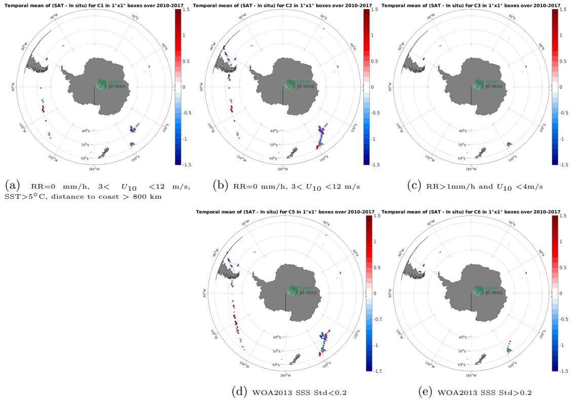
Figure 12: Temporal mean gridded over spatial boxes of size 1°x1° of \Delta SSS (SMOS SSS L2Q v331 - With FLAG (CMEMS-CATDS-CPDC) - TSG (GOSUD-Research-vessel)) for 5 different subdatasets corresponding to:RR=0 mm/h, 3 < U_{10} < 12 m/s, SST>5°C, distance to coast > 800 km (a), RR=0 mm/h, 3 < U_{10} < 12 m/s (b), RR>1mm/h and U_{10} < 4 m/s (c), WOA2013 SSS Std<0.2 (d), WOA2013 SSS Std>0.2 (e).
