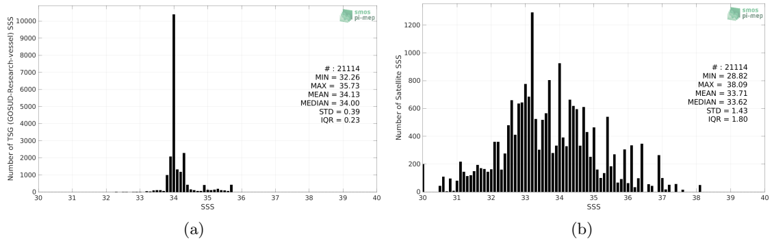
Figure 2: Histograms of SSS from TSG (GOSUD-Research-vessel) (a) and SMOS SSS L2Q v331 - With FLAG (CMEMS-CATDS-CPDC) (b) considering all match-up pairs per bins of 0.1 over the Roaring Forties and Furious Fifties Pi-MEP region and for the full satellite product period.
