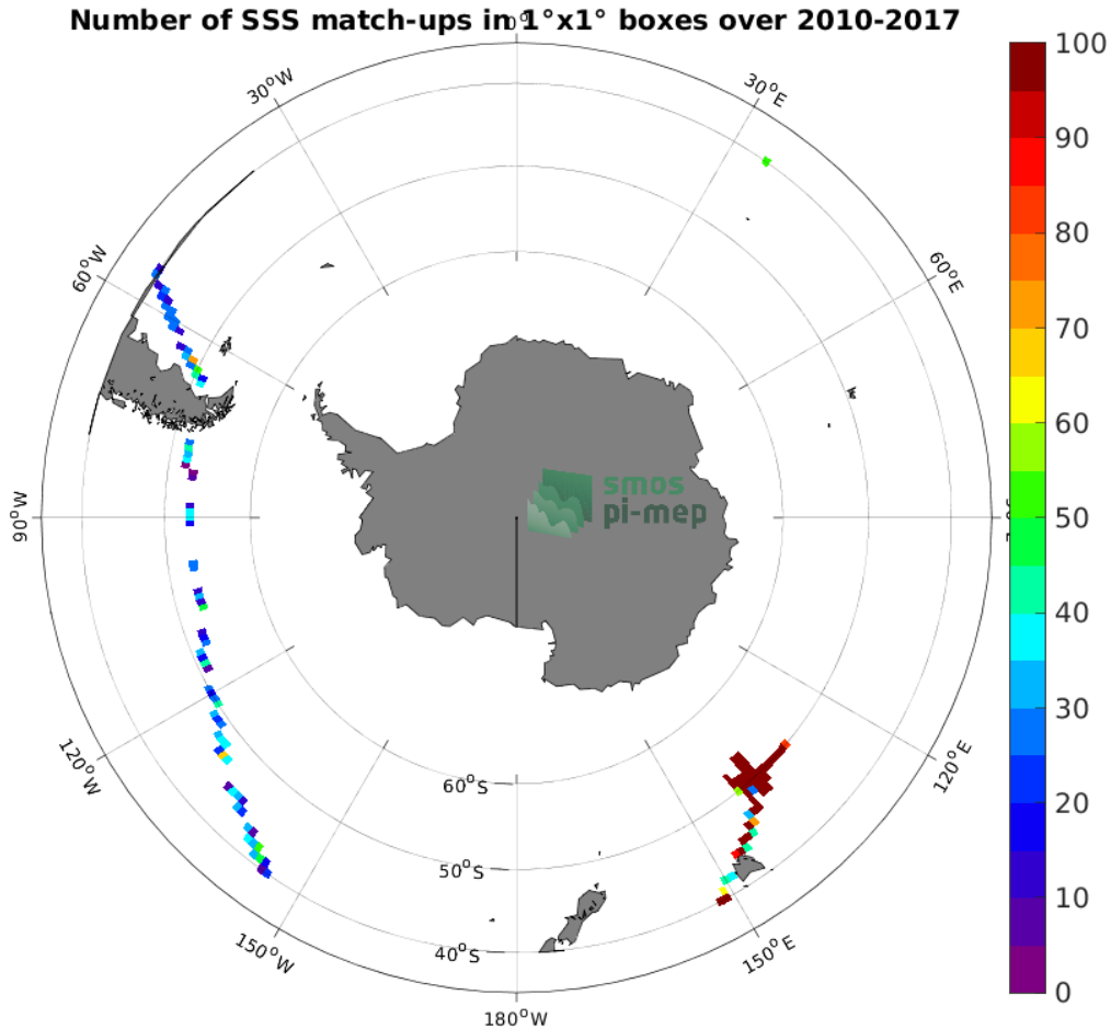
Figure 4: Number of SSS match-ups between TSG (GOSUD-Research-vessel) SSS and the SMOS SSS L2Q v331 - With FLAG (CMEMS-CATDS-CPDC) SSS product for the Roaring Forties and Furious Fifties Pi-MEP region over 1^\circ \times 1^\circ boxes and for the full satellite product period.
