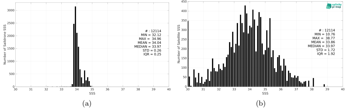
Figure 2: Histograms of SSS from Saildrone (a) and SMOS SSS L2Q v331 - With FLAG (CMEMS-CATDS-CPDC) (b) considering all match-up pairs per bins of 0.1 over the Roaring Forties and Furious Fifties Pi-MEP region and for the full satellite product period.
