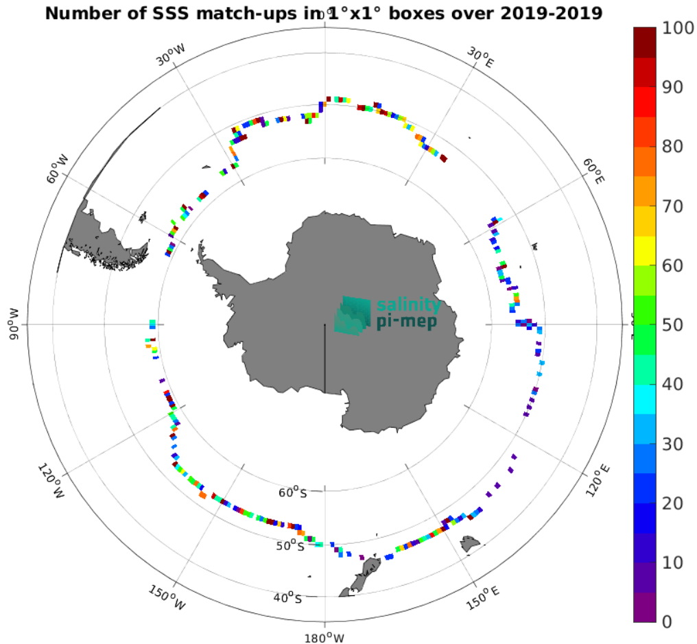
Figure 4: Number of SSS match-ups between Saildrone SSS and the SMOS SSS L2Q v331 - With FLAG (CMEMS-CATDS-CPDC) SSS product for the Roaring Forties and Furious Fifties Pi-MEP region over 1^\circ \times 1^\circ boxes and for the full satellite product period.
