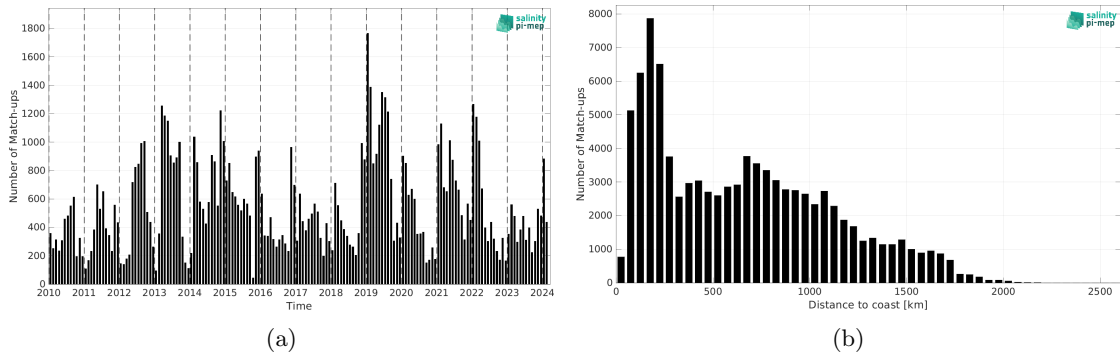
Figure 2: Number of match-ups between Marine mammals and SMOS SSS L2Q v331 - With FLAG (CMEMS-CATDS-CPDC) SSS as a function of time (a) and as function of the distance to coast (b) over the Roaring Forties and Furious Fifties Pi-MEP region and for the full satellite product period.
