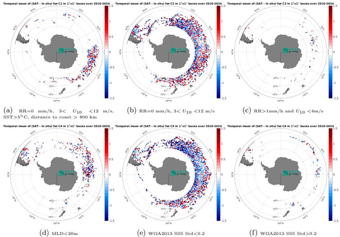
Figure 14: Temporal mean gridded over spatial boxes of size 1^\circ \times 1^\circ of \Delta SSS (SMOS SSS L2Q v331 - With FLAG (CMEMS-CATDS-CPDC) - Marine mammals) for 6 different subdatasets corresponding to:RR=0 mm/h, 3 < U_{10} < 12 m/s, SST>5°C, distance to coast > 800 km (a), RR=0 mm/h, 3 < U_{10} < 12 m/s (b), RR>1mm/h and U_{10} < 4 m/s (c),MLD<20m (d),WOA2013 SSS Std<0.2 (e),WOA2013 SSS Std>0.2 (f).
