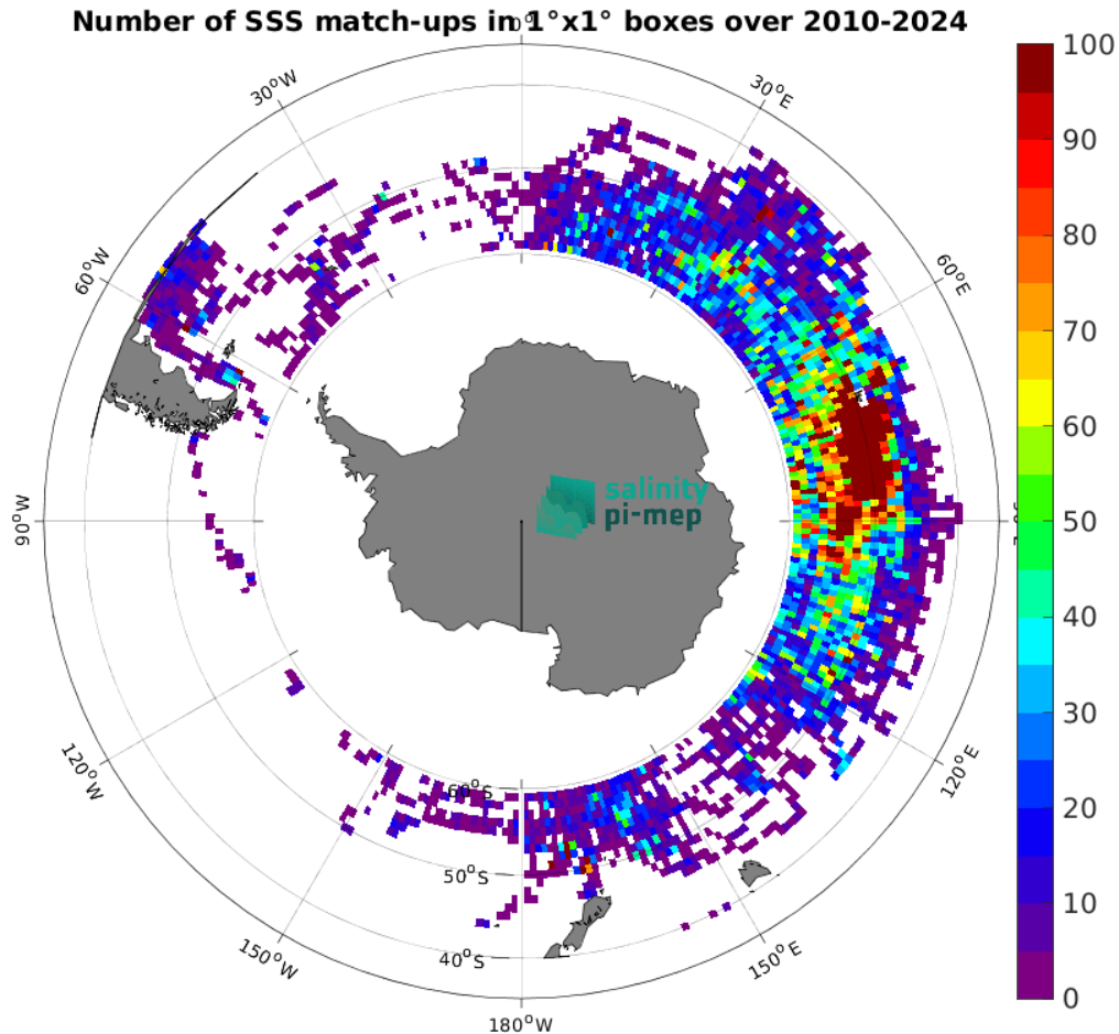
Figure 5: Number of SSS match-ups between Marine mammals SSS and the SMOS SSS L2Q v331 - With FLAG (CMEMS-CATDS-CPDC) SSS product for the Roaring Forties and Furious Fifties Pi-MEP region over 1^\circ \times 1^\circ boxes and for the full satellite product period.
