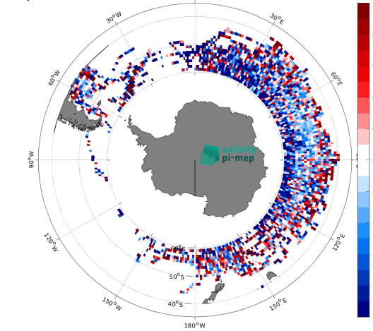
(e) MEAN( \Delta SSS) (Satellite - Marine mammals) 16
