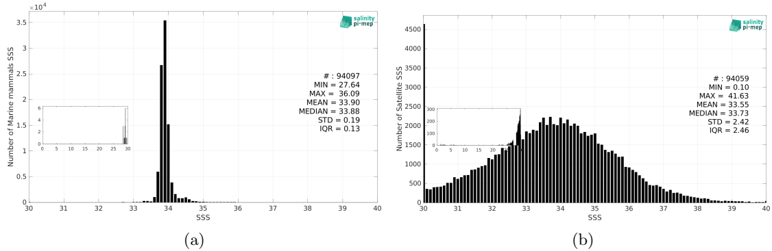
Figure 3: Histograms of SSS from Marine mammals (a) and SMOS SSS L2Q v331 - With FLAG (CMEMS-CATDS-CPDC) (b) considering all match-up pairs per bins of 0.1 over the Roaring Forties and Furious Fifties Pi-MEP region and for the full satellite product period.
