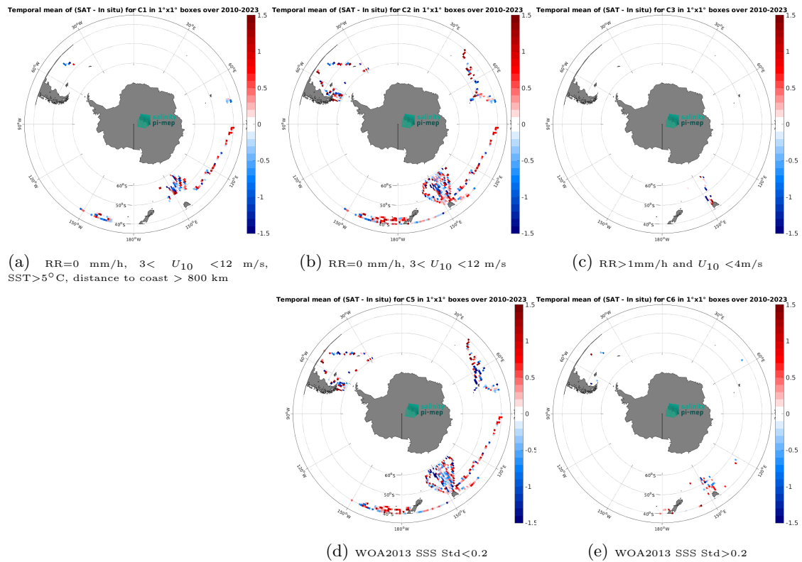
Figure 14: Temporal mean gridded over spatial boxes of size 1^\circ \times 1^\circ of \Delta SSS (SMOS SSS L2Q v331 - No FLAG (CMEMS-CATDS-CPDC) - TSG (LEGOS-DM)) for 5 different subdatasets corresponding to:RR=0 mm/h, 3 < U_{10} < 12 m/s, SST >5^\circ\text{C} , distance to coast > 800 km (a), RR=0 mm/h, 3 < U_{10} < 12 m/s (b), RR >1 mm/h and U_{10} < 4 m/s (c), WOA2013 SSS Std <0.2 (d), WOA2013 SSS Std >0.2 (e).
