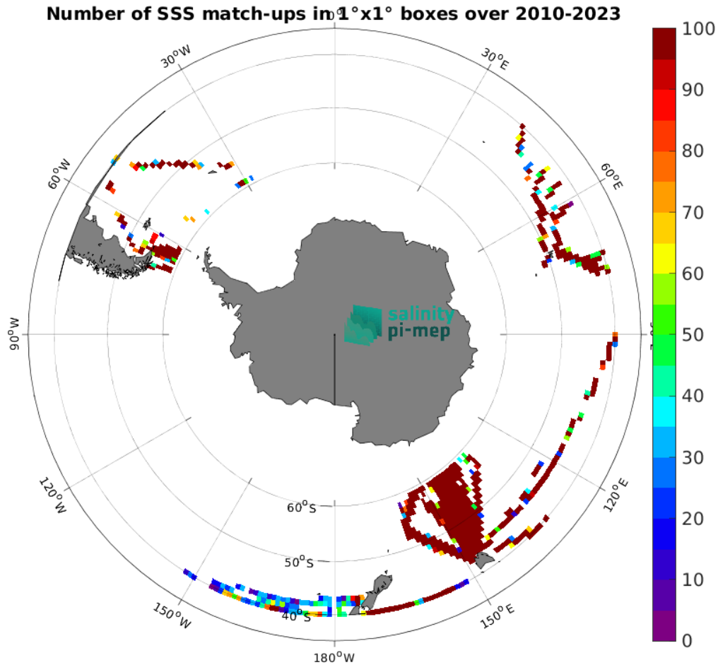
Figure 5: Number of SSS match-ups between TSG (LEGOS-DM) SSS and the SMOS SSS L2Q v331 - No FLAG (CMEMS-CATDS-CPDC) SSS product for the Roaring Forties and Furious Fifties Pi-MEP region over 1^\circ \times 1^\circ boxes and for the full satellite product period.
