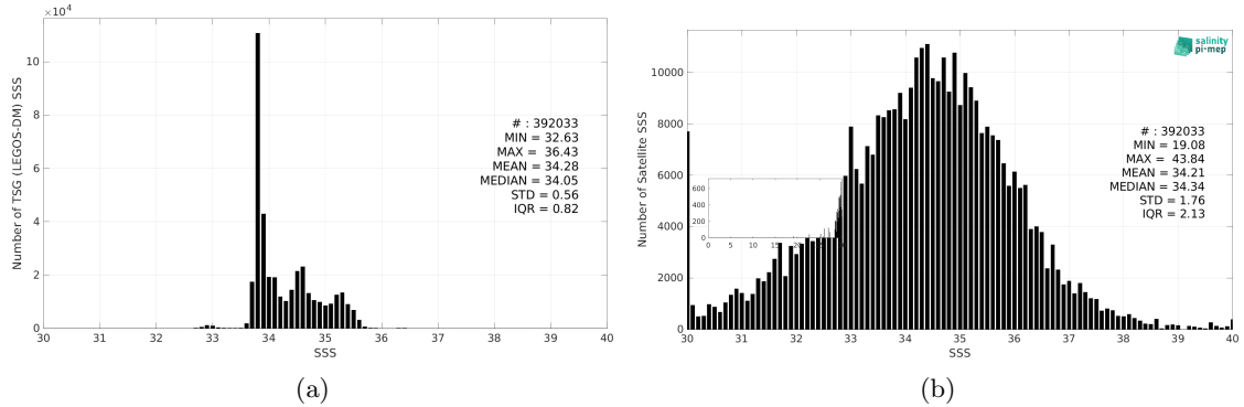
Figure 3: Histograms of SSS from TSG (LEGOS-DM) (a) and SMOS SSS L2Q v331 - No FLAG (CMEMS-CATDS-CPDC) (b) considering all match-up pairs per bins of 0.1 over the Roaring Forties and Furious Fifties Pi-MEP region and for the full satellite product period.
