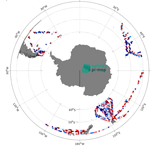
(e) MEAN( \Delta SSS) (Satellite - TSG (LEGOS-DM)) 16
