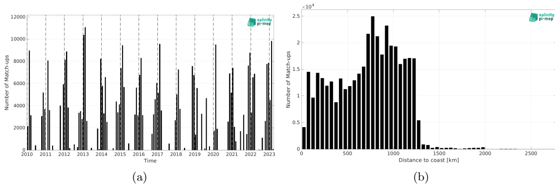
Figure 2: Number of match-ups between TSG (LEGOS-DM) and SMOS SSS L2Q v331 - No FLAG (CMEMS-CATDS-CPDC) SSS as a function of time (a) and as function of the distance to coast (b) over the Roaring Forties and Furious Fifties Pi-MEP region and for the full satellite product period.
