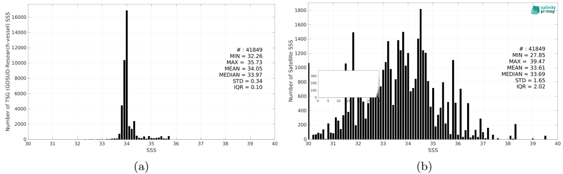
Figure 3: Histograms of SSS from TSG (GOSUD-Research-vessel) (a) and SMOS SSS L2Q v331 - No FLAG (CMEMS-CATDS-CPDC) (b) considering all match-up pairs per bins of 0.1 over the Roaring Forties and Furious Fifties Pi-MEP region and for the full satellite product period.
