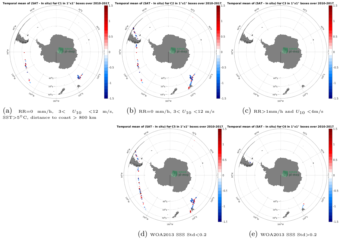
Figure 12: Temporal mean gridded over spatial boxes of size 1°x1° of \Delta SSS (SMOS SSS L2Q v331 - No FLAG (CMEMS-CATDS-CPDC) - TSG (GOSUD-Research-vessel)) for 5 different subdatasets corresponding to:RR=0 mm/h, 3 < U_{10} < 12 m/s, SST>5°C, distance to coast > 800 km (a), RR=0 mm/h, 3 < U_{10} < 12 m/s (b), RR>1mm/h and U_{10} < 4 m/s (c), WOA2013 SSS Std<0.2 (d), WOA2013 SSS Std>0.2 (e).
