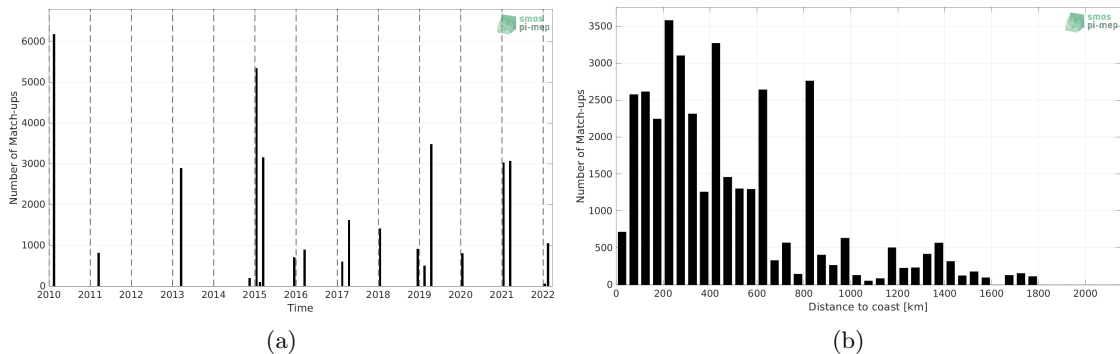
Figure 1: Number of match-ups between TSG (CSIC-UTM) and SMOS SSS L2Q v331 - No FLAG (CMEMS-CATDS-CPDC) SSS as a function of time (a) and as function of the distance to coast (b) over the Roaring Forties and Furious Fifties Pi-MEP region and for the full satellite product period.
