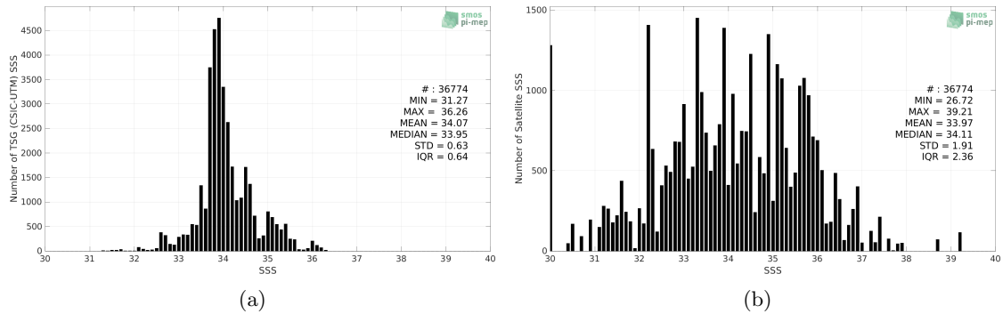
Figure 2: Histograms of SSS from TSG (CSIC-UTM) (a) and SMOS SSS L2Q v331 - No FLAG (CMEMS-CATDS-CPDC) (b) considering all match-up pairs per bins of 0.1 over the Roaring Forties and Furious Fifties Pi-MEP region and for the full satellite product period.
