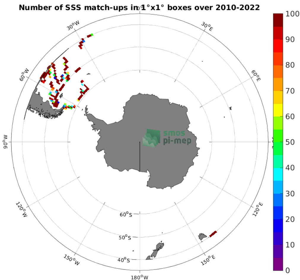
Figure 4: Number of SSS match-ups between TSG (CSIC-UTM) SSS and the SMOS SSS L2Q v331 - No FLAG (CMEMS-CATDS-CPDC) SSS product for the Roaring Forties and Furious Fifties Pi-MEP region over 1^\circ \times 1^\circ boxes and for the full satellite product period.
